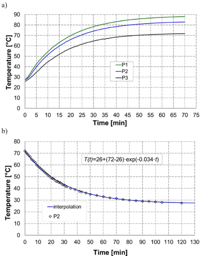
Fig. 4. Temperature changes on the surface of the shock absorber (left – heating, right – cooling)
