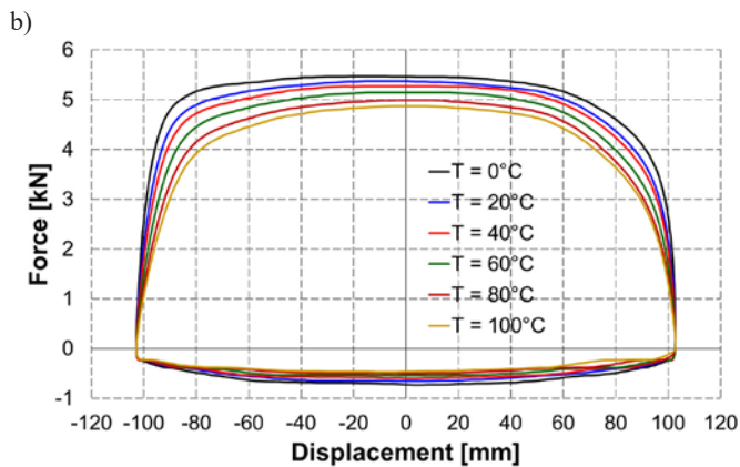
Fig. 5. Influence of the temperature on the force-displacement characteristics of the shock absorber (left – amplitude 50 mm, right – amplitude 100 mm)
