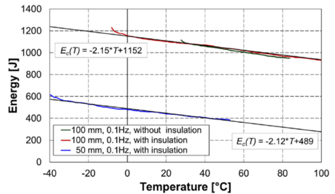
Fig. 7. Energy dissipated in one cycle
