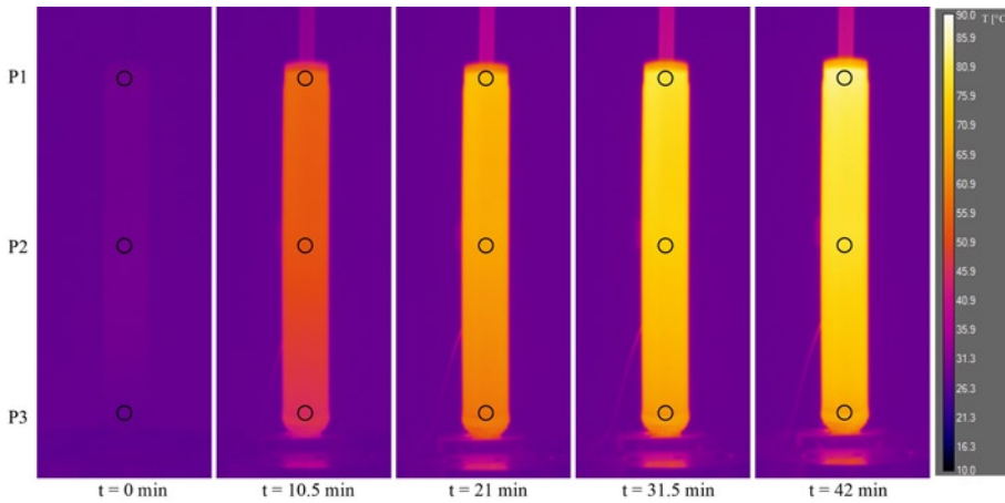
Fig. 3. Selected temperature distributions on the walls of the shock absorber
