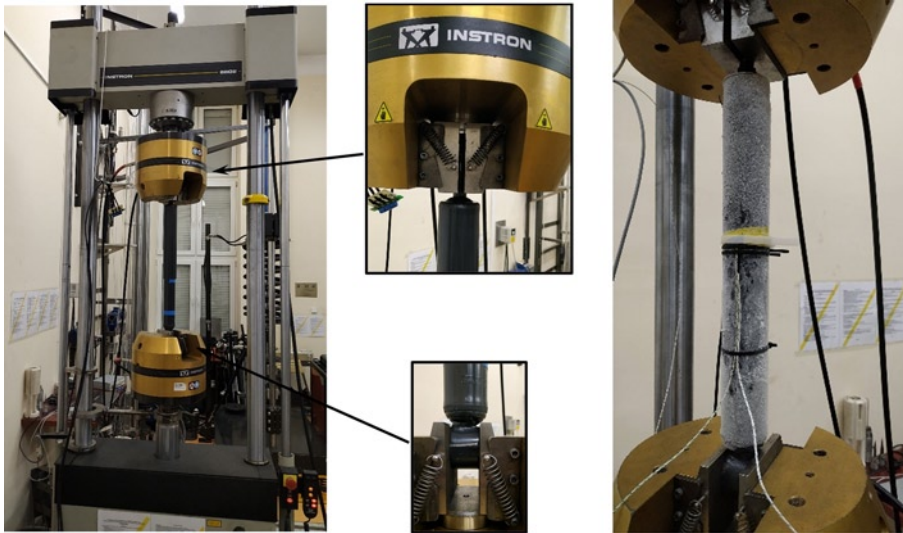
Fig. 1. The testing stand
