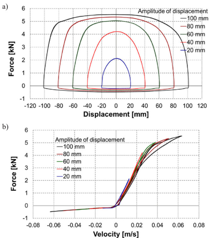
Fig. 2. Force-displacement and force-velocity characteristics of the shock absorber
