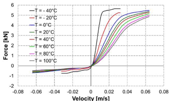
Fig. 6. Temperature influence on the damping characteristic curves of the shock absorber
