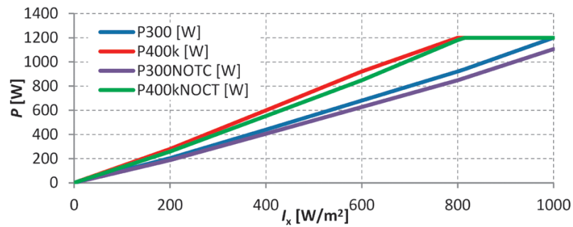
Fig. 10. The temperature impact on the active power output of the PV micro plant with rated power capacity P_n = 1200 W, as a function of constant irradiance I_x , 1650 h
