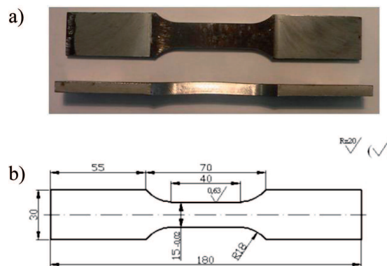
Fig. 2. Photo (a) and schematic illustration (b) of samples cut in the circumferential direction
