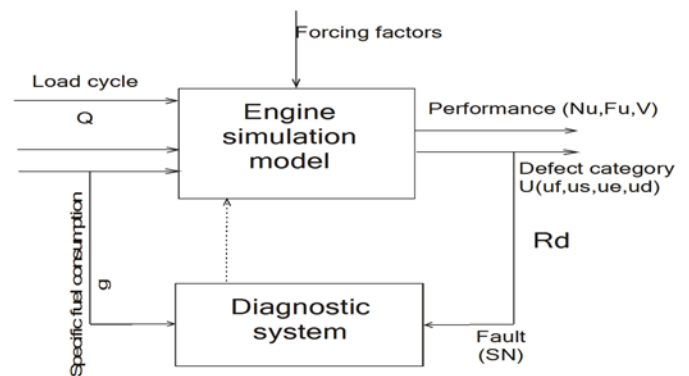
Fig. 1. Diagnostic diagram of a wheeled tractor based on the proposed mechatronic system for monitoring the condition of wheeled tractor (MSMC), where: g – specific fuel consumption, N_U – pulling power; pulling power; F_U – pulling force; V – speed; SN – fault, Q – load; u – defect category [13]
