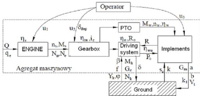
Fig. 3. Structural diagram of a wheeled tractor in the process of monitoring operating parameters [11]: \beta – ground inclination (slope), \delta – slip ratio of drive wheels, \phi – coefficient of tractive adhesion, \eta_m – mechanical efficiency, \eta_o – tractive efficiency (total), \eta_s – engine efficiency, \eta_u – traction efficiency, \eta_{wu} – traction efficiency rating, a – width of implement, b – depth of implement, f – coefficient of rolling resistance, M_w – PTO torque, n_w – PTO rotational speed, \eta_w – PTO efficiency, g_e – specific fuel consumption, G_c – tractor mass, G_m – implement mass, i_c – overall gear ratio, k – soil strength, k_1 – rolling resistance of implement, M_k – driving torque, M_s – net torque, N_e – effective power, N_k – driving power, N_n – nominal power output, n_s – engine rotational speed, P_n – driving force, Q – fuel consumption per hour, s_2 – presence of field stones, u_1 – fuel dose, u_2 – applied gear ratio, u_3 – operating mode, Y_k – load on drive wheels, V_t – operating speed of implement operation, R – resistance of implement, R_0 – resistance in the drive, PTO – power takeoff
