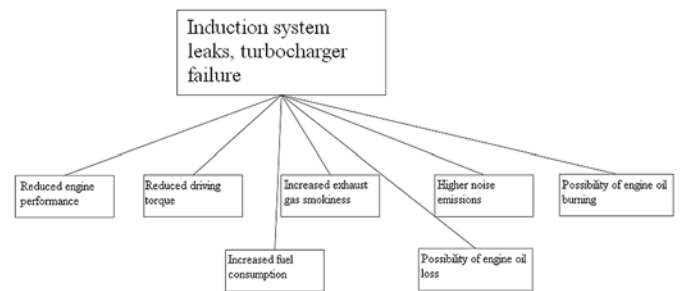
Fig. 9. Diagnostic symptoms of induction system leaks and turbocharger failure
