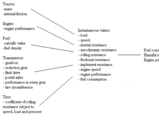
Fig. 2. Correlations between a tractor's technical parameters in a defect simulation model
