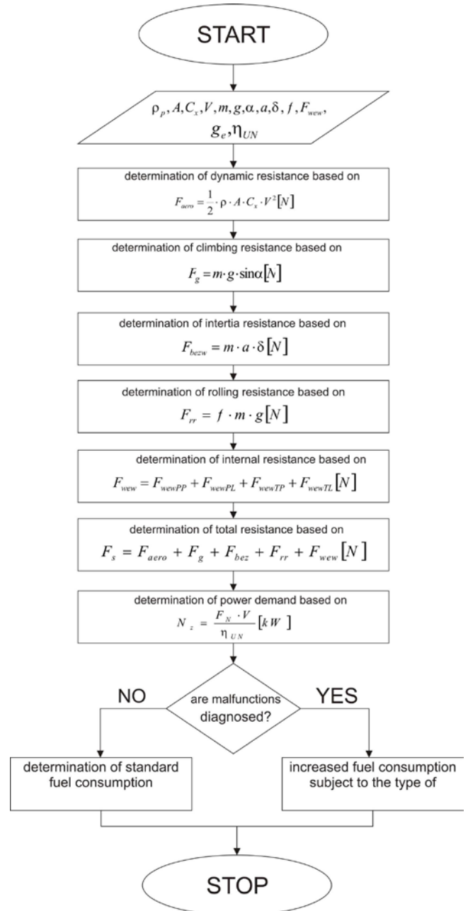
Fig. 4. An algorithm for determining fuel consumption in simulated tractor malfunctions g_e – specific fuel consumption, \rho_p – fuel density, \rho – air density, A – area of the tractor's front face, C_x – coefficient of aerodynamic drag, V – velocity, m – mass, g – gravitational acceleration, \alpha – ground inclination, a – acceleration, \delta – rotational mass coefficient, f – rolling resistance coefficient, F_{wew} – internal resistance on each wheel, \eta_{UN} – power transmission efficiency.
