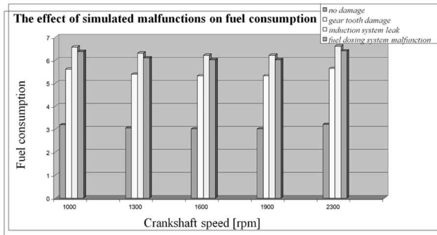
Fig. 12. Correlations between changes in fuel consumption and the simulated malfunctions: no damage, gear tooth damage, induction system leak, fuel dosing system malfunction.
