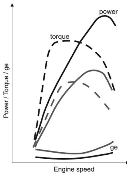
Fig. 10. The effect of fuel dosing system malfunctions on engine performance (black – optimally functioning engine, red – malfunctioning engine)
