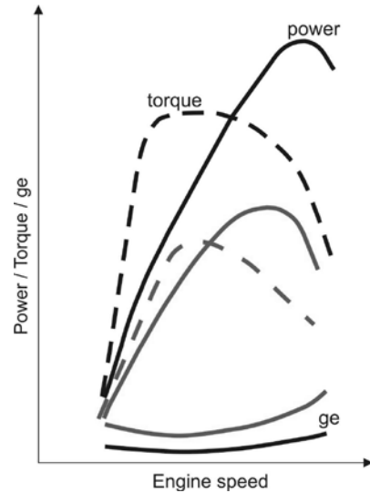
Fig. 7. The effect of induction system leaks and turbocharger failure on engine performance
