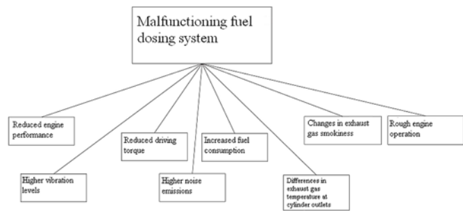
Fig. 11. Diagnostic symptoms of fuel dosing system malfunctions
