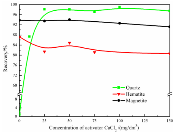
Fig. 6. Flotation recoveries as a function of \text{CaCl}_2 concentration, at 25^\circ\text{C} . (Quartz flotation: \alpha -BLA 75 \text{ mg}/\text{dm}^3 , pulp pH=11.5. Hematite flotation: \alpha -BLA 125 \text{ mg}/\text{dm}^3 , pulp pH=6.45. Magnetite flotation: \alpha -BLA 125 \text{ mg}/\text{dm}^3 , pulp pH =6.97)
