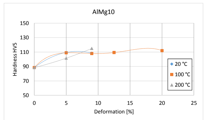
Fig. 20. The evolution of the AlMg10 hardness in terms of the cold rolling temperature and the given deformation
