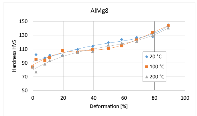
Fig. 18. The evolution of the AlMg8 hardness in terms of the cold rolling temperature and the given deformation
