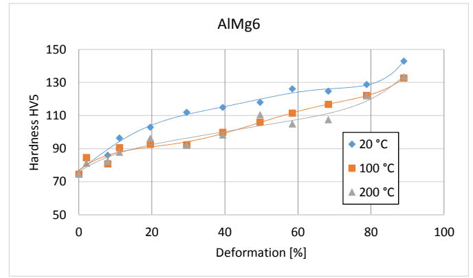
Fig. 16. The evolution of the AlMg6 hardness in terms of the cold rolling temperature and the given deformation
