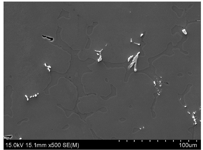
Fig. 4. Microstructure of the casted AlMg9 alloy
