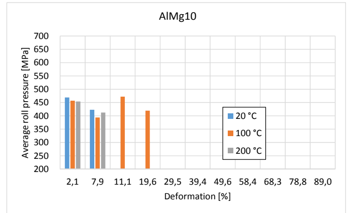
Fig. 12. The influence of the temperature and given strain during the cold rolling of AlMg10 in terms of an average unit pressure
