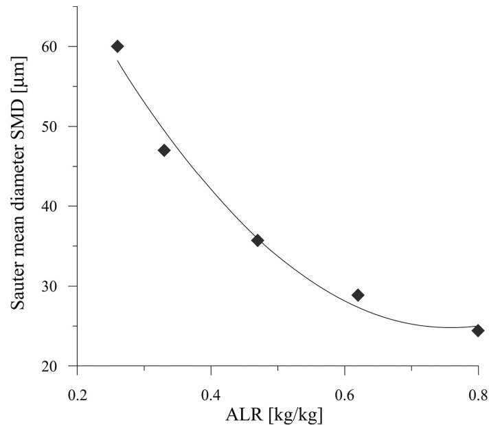
Fig. 4. Mean diameter of droplets of dispersed spray as a function of ALR
