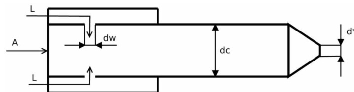
Fig. 3. Schematic diagram of an atomiser with characteristic dimensions marked
