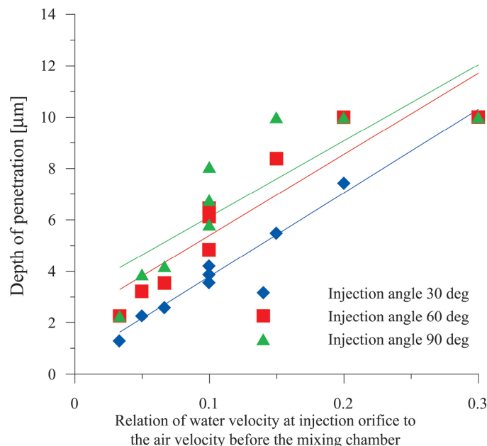
Fig. 2. Depth of penetration 30 mm from the injection point as a function of ratio of water velocity at injection orifice to the air velocity in central pipe before the mixing chamber ( d_w=0.2 mm p_c=6 bar)
