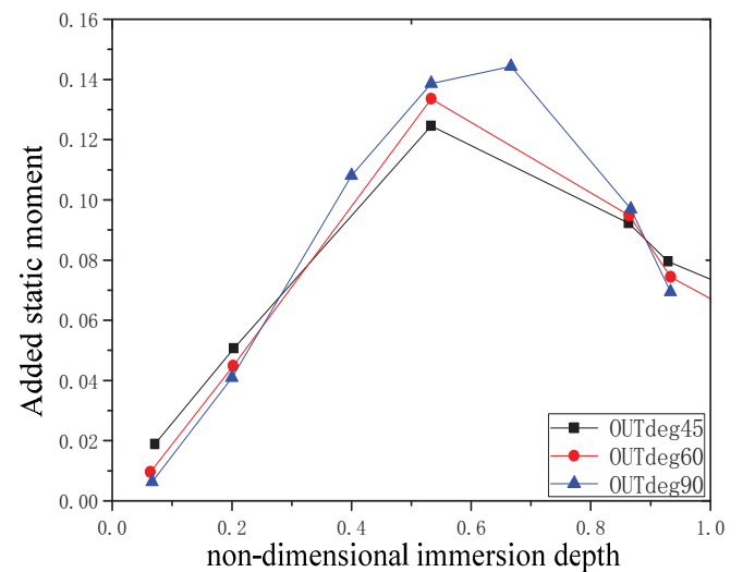
Fig. 12. Added static moment
