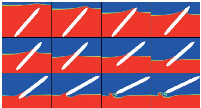
Fig. 13. Numerical simulated results of water-exit motion
