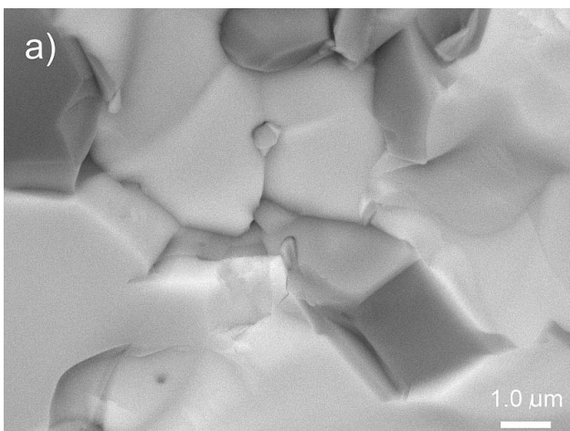
Fig. 4. BSE images of the microstructure of fracture of the BFN-F samples: FSc sample (a) and SPSc sample (b)
