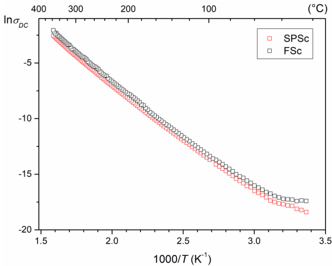
Fig. 6. The \ln\sigma_{DC}(1000/T) dependences of the BFN-F composites
