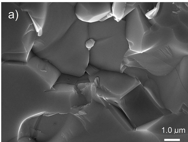
Fig. 3. SEM images of the microstructure of fracture of the BFN-F samples: FSc sample (a) and SPSc sample (b), at the standard SB mode
