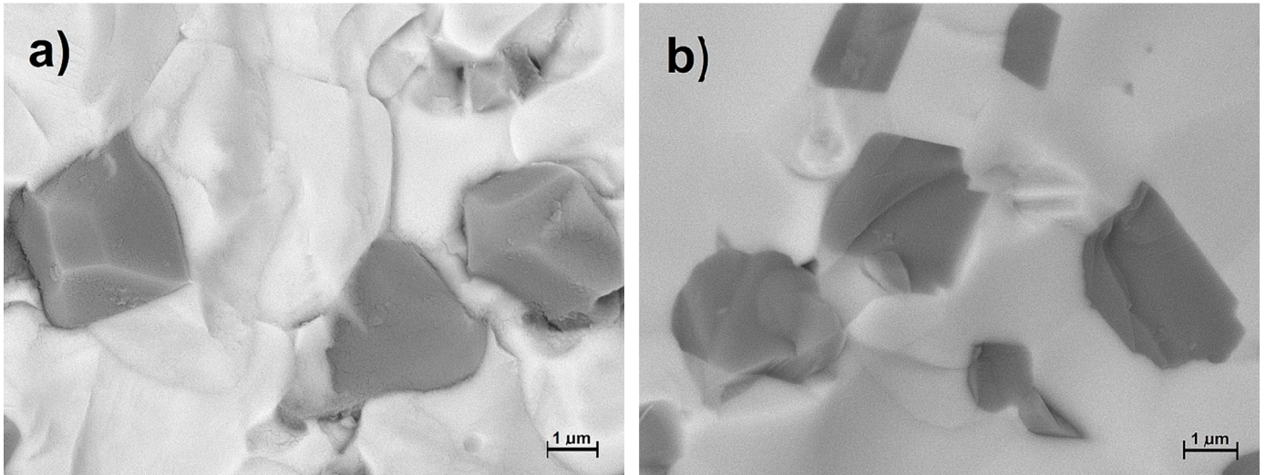
Fig. 5. BS images of the microstructure of fracture of magnetolectric PFN-ferrite (a) and BFN-ferrite (b) composites
