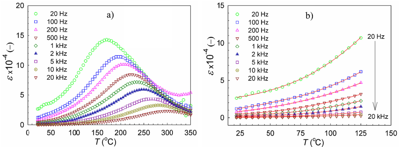
Fig. 9. Temperature dependencies of dielectric constant \epsilon for BFN-ferrite composite (a), solid lines represent theoretical curves (b)
