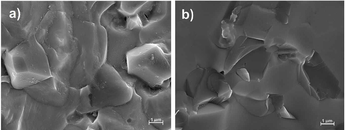
Fig. 4. SEM images of the microstructure of fracture of magnetolectric PFN-ferrite (a) and BFN-ferrite (b) composites (at the standard SB mode)
