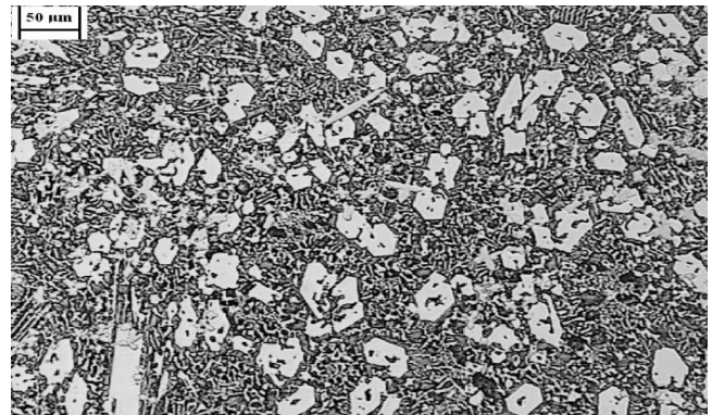
Fig. 1. Chromium carbides on the top of surface layer
