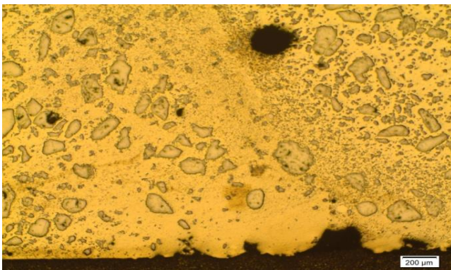
Fig. 5. Lack of fusion between the layer
