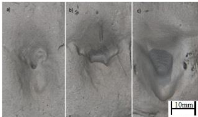
Fig. 15. Phases erosive wear abrasive welds
