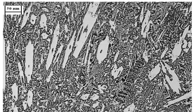
Fig. 2. Chromium carbides in the middle of surface layer
