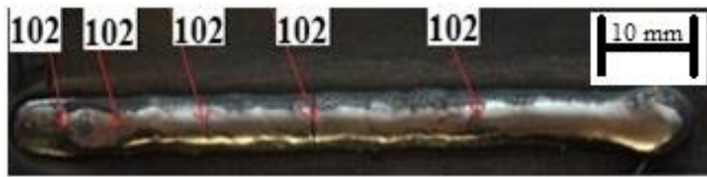
Fig. 10. Craks in the single bead with describe according to norm PN EN ISO 6520-1
