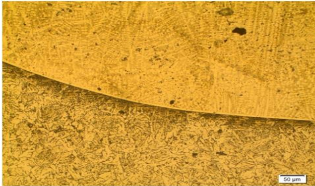
Fig. 4. Cavities over the fusion line
