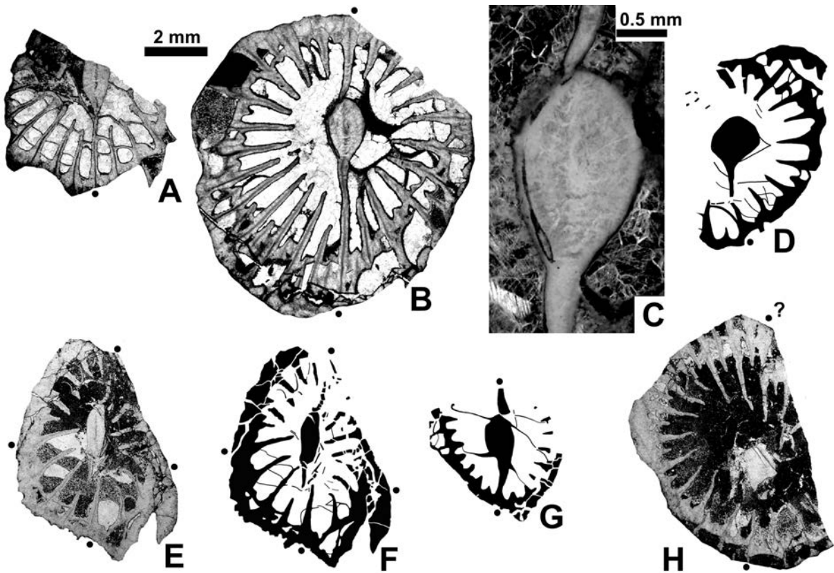
Text-fig. 6. Protokionophyllum facilis Vassilyuk, 1983. Transverse thin sections. A–C – Specimen UAM-Tc.Don.1/346. Holotype. A – late neanic or early mature growth stage; B – mature growth stage; C – pseudocolumella (enlarged from B). D – Specimen UAM-Tc.Don.1/347. Hypotype. Mature growth stage. E, F – Specimen UAM-Tc.Don.1/351. Hypotype. Late neanic growth stage (F – drawing on E). G – Specimen UAM-Tc.Don.1/349. Hypotype. Late neanic growth stage. H – Specimen UAM-Tc.Don.1/350. Hypotype. Lower part of calice. For stratigraphic positions see text. Cardinal, counter and alar septa marked by black dots when recognisable. Scale bar between A and B corresponds to all images except C.
