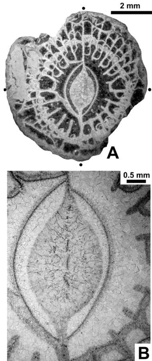
Text-fig. 11. Protokionophyllum sp. 2. Specimen UAM-Tc.Don.1/364. A – transverse section, mature growth stage; B – pseudocolumella (enlarged from A). For stratigraphic position see text. Protosepta and alar septa marked by black dots.
