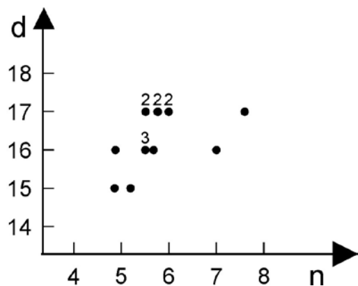
Text-fig. 22. Colligophyllum dobroljubovae (Vassilyuk, 1960). N:d value where n = number of septa and d = corallite diameter. Numbers above black dots correspond to number of corallites with given value.
