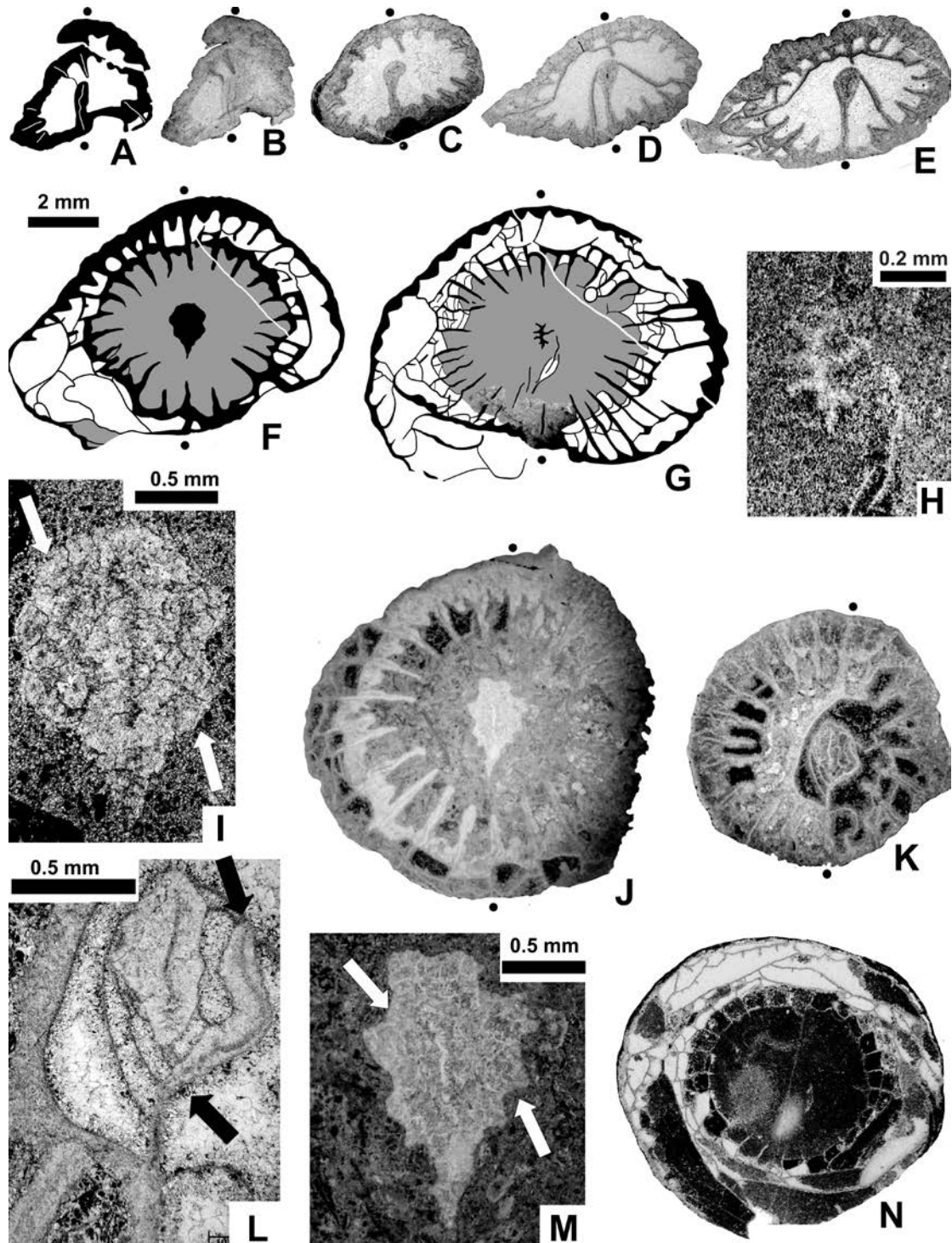
Text-fig. 15. Krynkaphyllum multiplexum sp. nov. A-F, H-N. Transverse thin sections. A-I – Specimen UAM-Tc.Don.1/368. Possible paratype. A-E – immature growth stage (A – drawing on B); F, G – calice (F – drawing on thin section; G – drawing on peel); H – pseudocolumella in middle part of calice; free septal lamellae attached to median lamella (enlarged from G); I – lower part of calice; innermost parts of tabulae, with septal lamellae incorporated (arrows), closely fit pseudocolumella (enlarged from F). J-M – Specimen UAM-Tc.Don.1/369. Possible paratype. Mature growth stage. J – calice; K – 5 mm below calice; L – inner margin of cardinal septum strongly thickened (arrows), surrounding pseudocolumella free from both protosepta (enlarged from K); M – pseudocolumella; last tabula with septal lamellae incorporated, closely fits median lamella elongated towards cardinal septum (enlarged from J). N – Specimen UAM-Tc.Don.1/370. Possible paratype. Calice. For stratigraphic positions see text. Protosepta marked by black dots when recognisable. Scale bar between A and F corresponds to images A-G, J, K, N.
