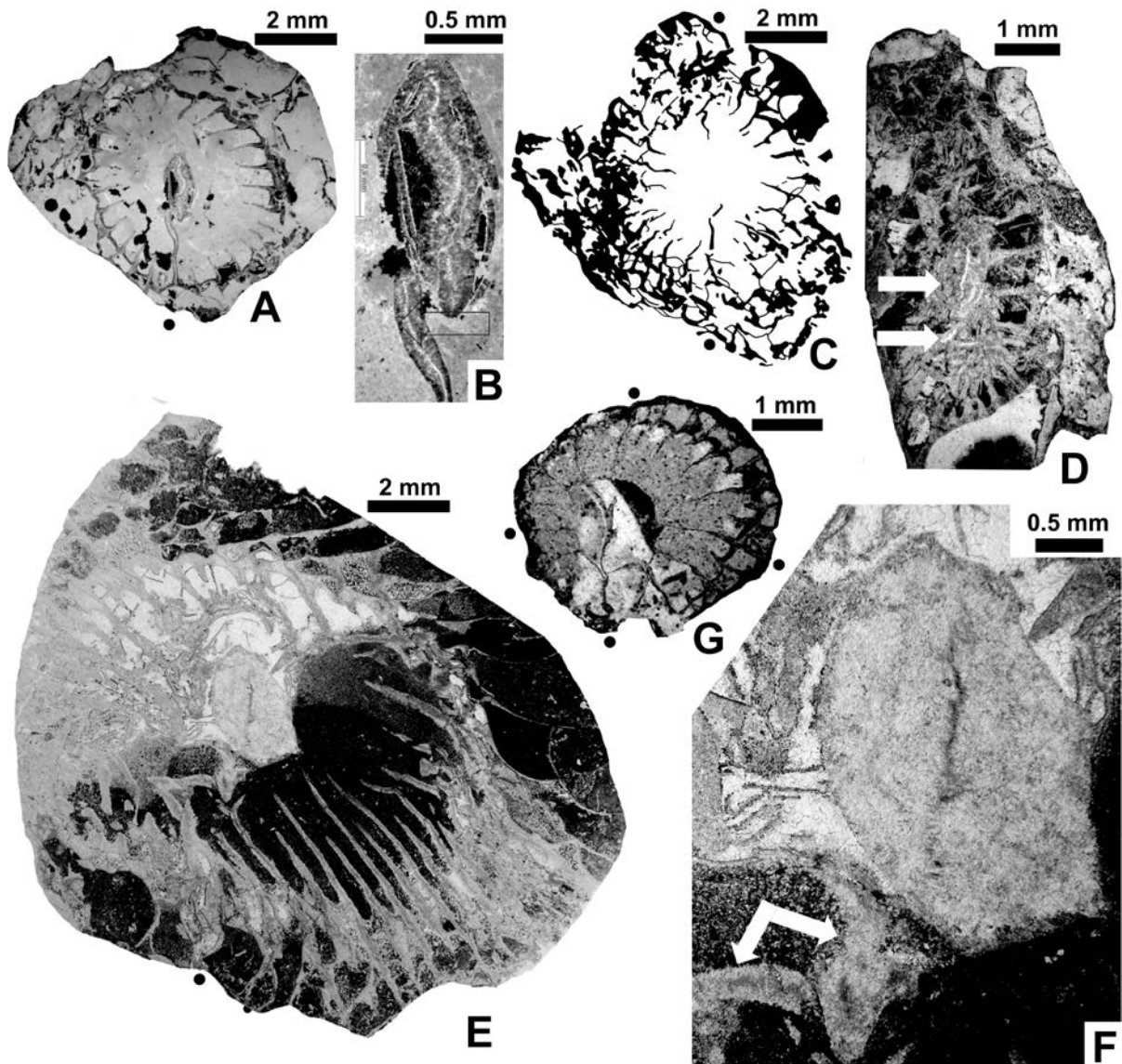
Text-fig. 10. Protokionophyllum sp. 1. Transverse thin sections. A, B – Specimen UAM-Tc.Don.1/360. A – mature growth stage; B – pseudo-columella and long cardinal septum (enlarged from A). C – Specimen UAM-Tc.Don.1/361. Mature growth stage (drawing on thin section image). D–F – Specimen UAM-Tc.Don.1/362. D – early mature growth stage; pseudo-columella (upper arrow) united with cardinal septum (lower arrow); E – mature growth stage; F – broken cardinal septum (white arrows) meets monoseptal pseudo-columella. G – Specimen UAM-Tc.Don.1/363. Lower part of calice; mature (?) growth stage. For stratigraphic positions see text. Protosepta and alar septa marked by black dots when recognisable.
