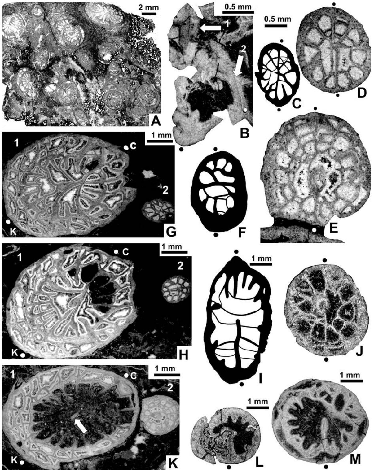
Text-fig. 19. Colligophyllum dobrolyubovae (Vassilyuk, 1960). Transverse thin sections except when stated otherwise. Type specimen UAM-Tc. Don.1/375 (= 1405/12; Vassilyuk 1960, p. 103). A – gregarium; B – two poorly preserved corallites in brephic (corallite 1) and early neanic (corallite 2) growth stage; C–E – successive sections from neanic to early mature growth stage of one corallite (enlarged from 18G, H, K, corallite 2); F, I, J, L, M – four immature corallites; G, H, K – successive transverse sections of two corallites from mature growth stage to calice with free pseudocolumella (arrows) in corallite 1; corallite 2 as described above. For stratigraphic position see text. Cardinal and counter septa marked by black or white dots when recognisable. Scale bar between B and D corresponds to images C–F, J.
