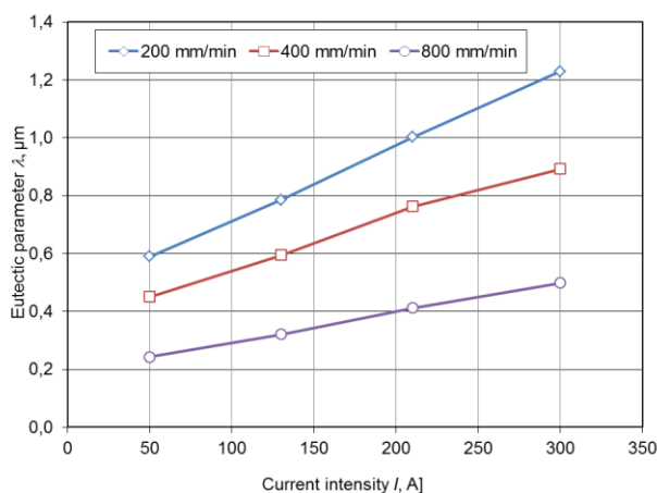
Fig. 6. The effect of the electric arc current intensity and the speed of scanning with electric arc on values of the parameter \lambda characterizing the cementite eutectic formed in remeltings made on nodular cast iron plate castings
