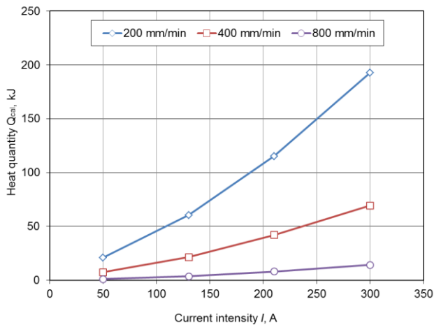
Fig. 3. The effect of the electric arc current intensity and the speed of scanning with electric arc on the quantity of heat introduced to the test casting
