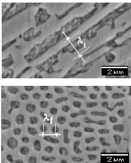
Fig. 1. Determination of structural parameter \lambda in lamellar and fibrous cementite eutectic
