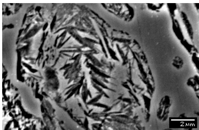
Fig. 2. Microstructure of a remelting in which austenite was subject to partial transformation into martensite in the course of cooling down to ambient temperature
