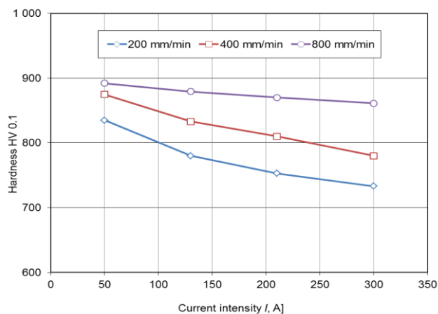
Fig. 7. The effect of the electric arc current intensity and the speed of scanning with electric arc on hardness of remeltings made on nodular cast-iron plate casting
