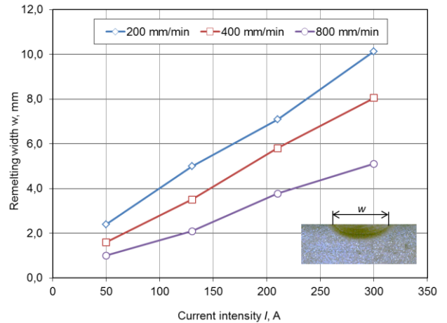
Fig. 4. The effect of the electric arc current intensity and the electric arc scanning speed on width of remeltings made on a plate cast from nodular cast iron
