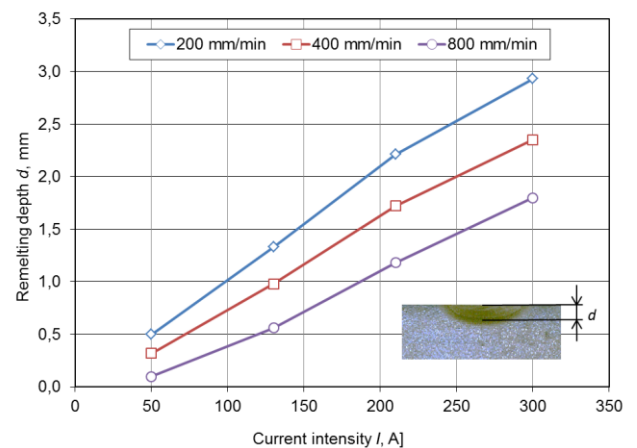
Fig. 5. The effect of the electric arc current intensity and the electric arc scanning speed on depth of remeltings made on a plate cast from nodular cast iron
