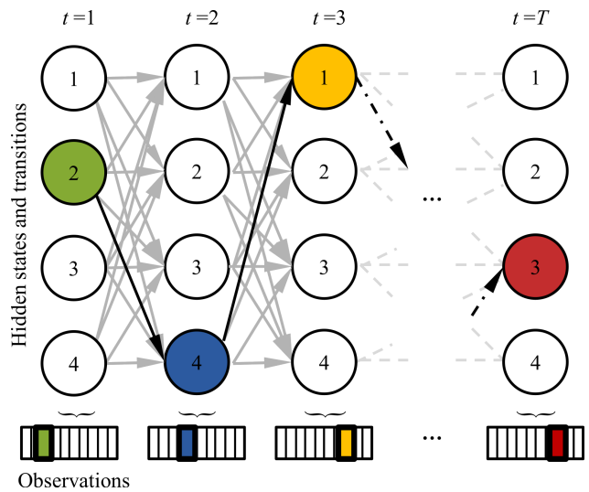
Fig. 2. Ergodic Hidden Markov Model – hidden state transition.
