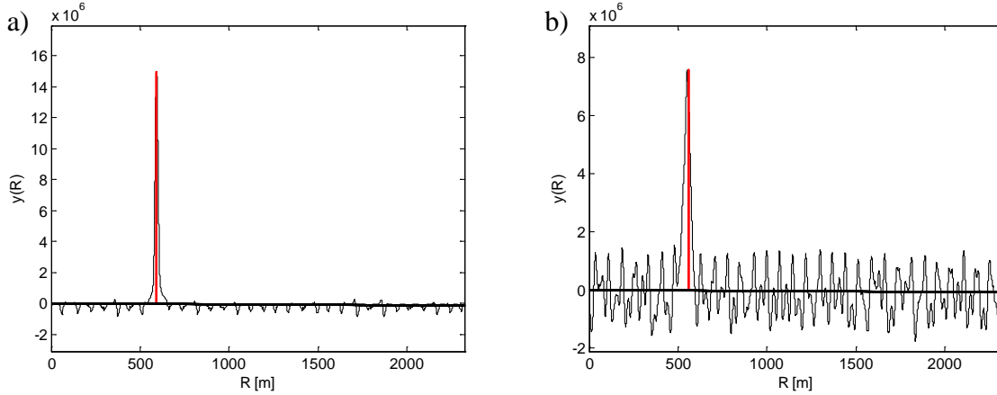
Fig. 16. The effect of speed on output signal: a) v = 2 m/s, b) v = 10 m/s. ( f_0 = 10 kHz, B = 2 kHz, B_e = 0.4 kHz, p = 0.2 , N = 5 , T_e = 0.1 s, p = 0.2 ).
