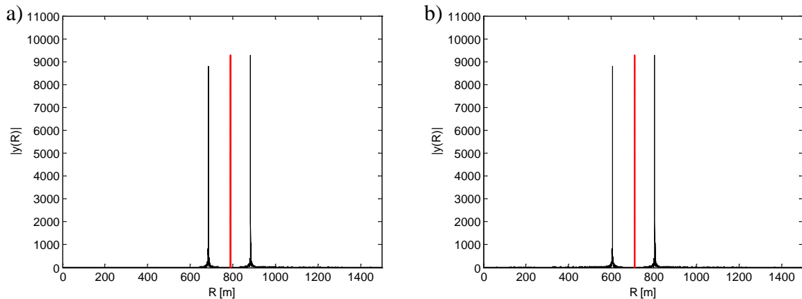
Fig. 2. Output signals ( v = 10 m/s): a) – first measurement cycle, b) – fifth measurement cycle.
