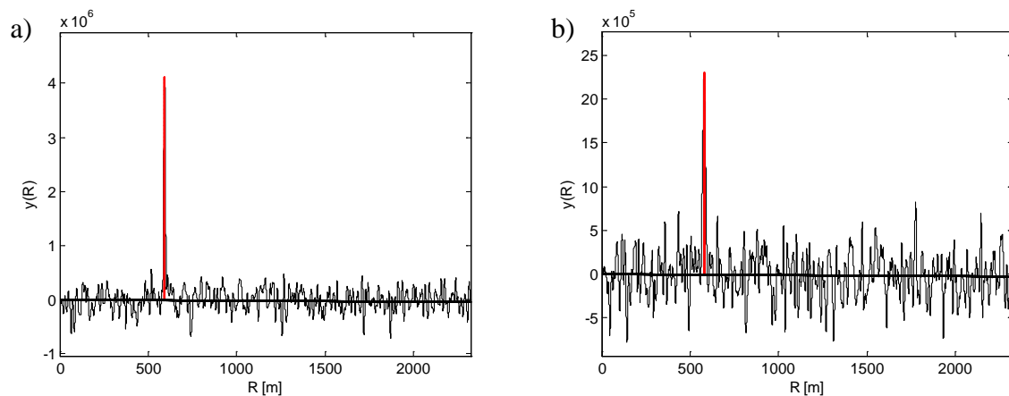
Fig. 17. The effect of target speed on output signal parameters for \text{SNR}_i = 0 dB: a) v = 2 m/s, b) v = 5 m/s. ( f_0 = 10 kHz, B = 2 kHz, B_e = 0.4 kHz, N = 5 , T_e = 0.1 s, T_a = 10 ms).
