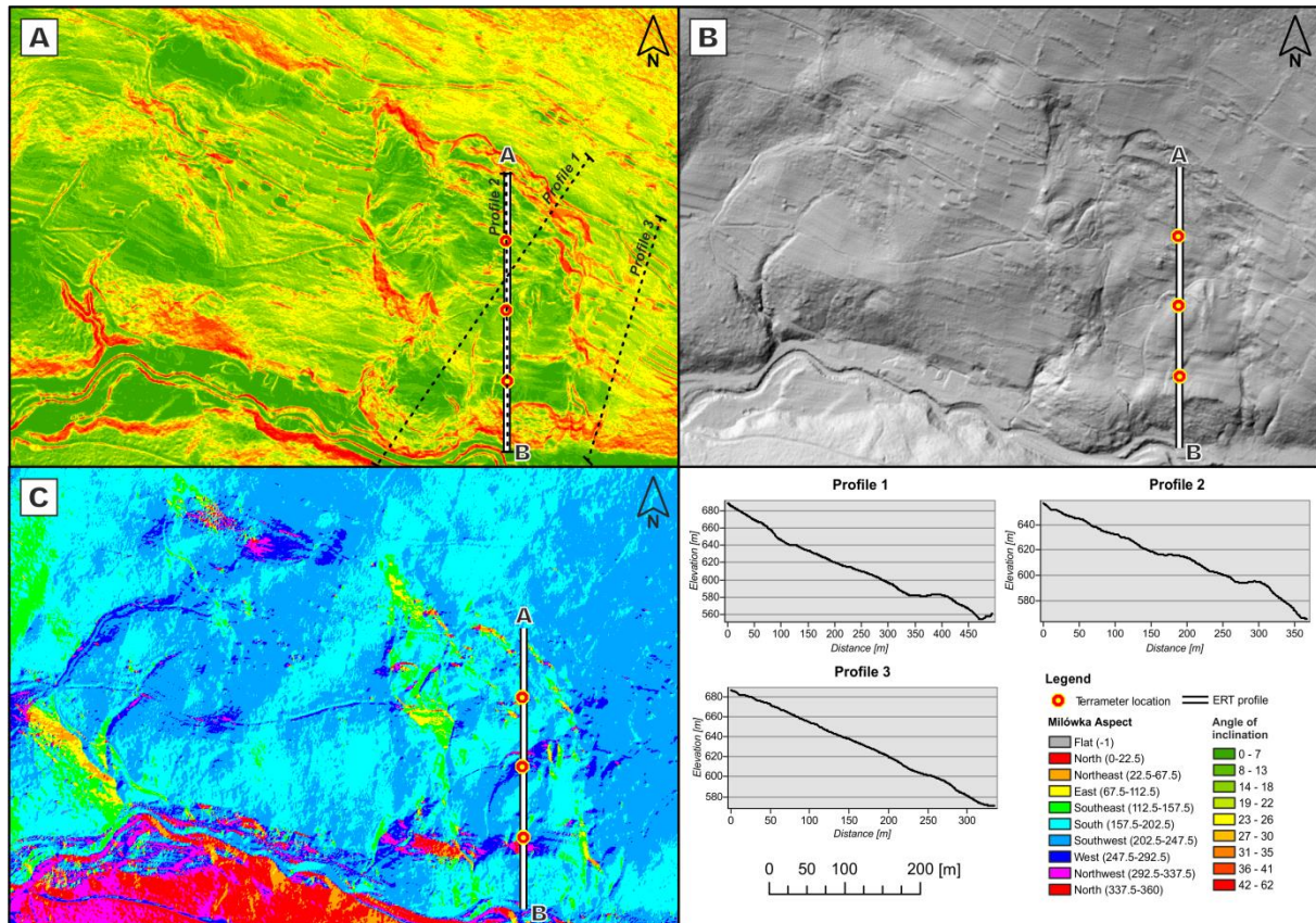
Fig.3. Raster maps of parameters of Milówka landslide. (A) Slope inclination in [°]. (B) Hillshade map. (C) Aspect map.
