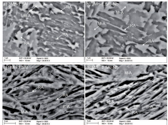
Fig. 3. SEM micrographs showing the morphology of structural constituents in 3Mn-1.5Al (a), 3Mn-1.5Al-Nb (b), 5Mn-1.5Al (c) and 5Mn-1.5Al-Nb steels (d); RA – retained austenite, \alpha_B – bainitic ferrite, M-A – martensite-austenite constituents, B-A – bainite-austenite constituents
