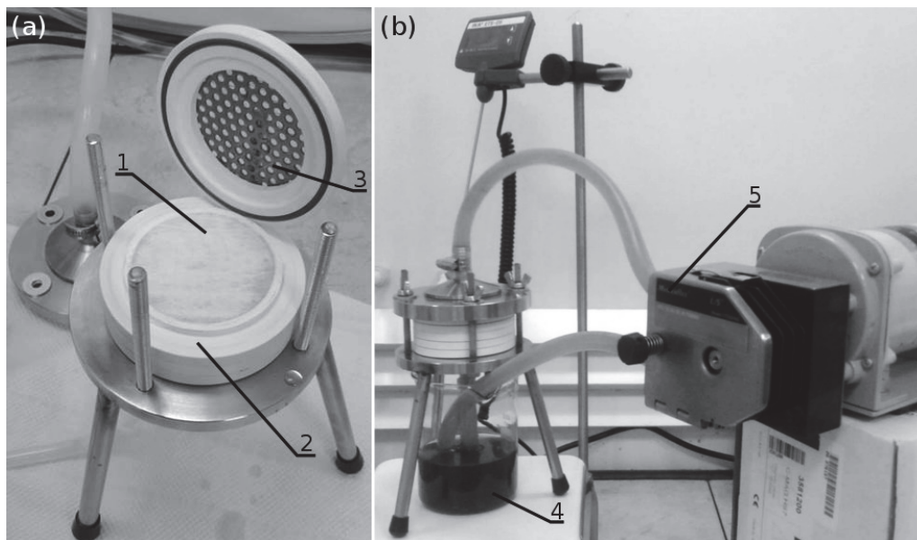
Fig. 2. Equipment used for water filtration tests: housing for filter media (a) and setup during operation (b); 1 - sample of filter media, 2 - spacer with seal, 3 - support for nonwovens, 4 - test dispersion, 5 - peristaltic pump
