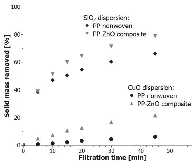
Fig. 9. Solid mass removed from aqueous dispersions of SiO 2 and CuO particles during 60 min of filtration
