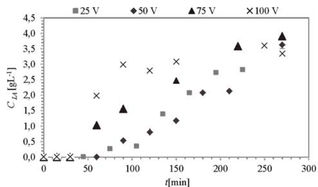
Figure 3. LA concentration in the right (III) chamber in time of electrodialysis. The initial concentration in the middle (feed) chamber (II) C_{0,II\_25V} = 7.42 \text{ g L}^{-1} ; C_{0,II\_50V} = 7.43 \text{ g L}^{-1} ; C_{0,II\_75V} = 7.25 \text{ g L}^{-1} ; C_{0,II\_100V} = 7.48 \text{ g L}^{-1}
