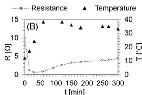
Figure 6. An example of the resistance, temperature and LA concentration in chamber III profile in time (electro dialysis at 100 V)
