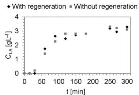
Figure 7. The profile of LA concentration in chamber III (the process at 50 V) using the membranes with and without regeneration
