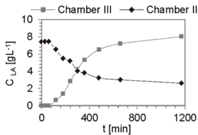
Figure 4. The change of LA concentration during electro dialysis carried out at 25 V
