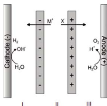
Figure 1. Scheme of an electro dialysis set
