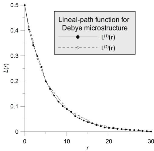
Fig. 7. Lineal-path function for Debye microstructure versus distance r given in pixels
