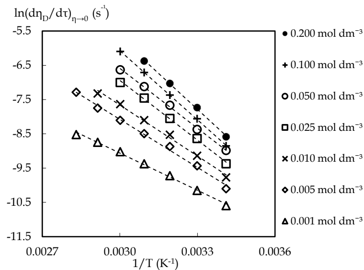
Fig. 7. Evaluation of the values of apparent activation energy for the studied concentrations of nitric acid
