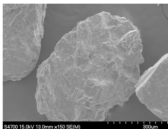
Fig. 3. SEM picture of dolomite particles (- 0.40 + 0.50 mm) - detailed picture of single particle.
