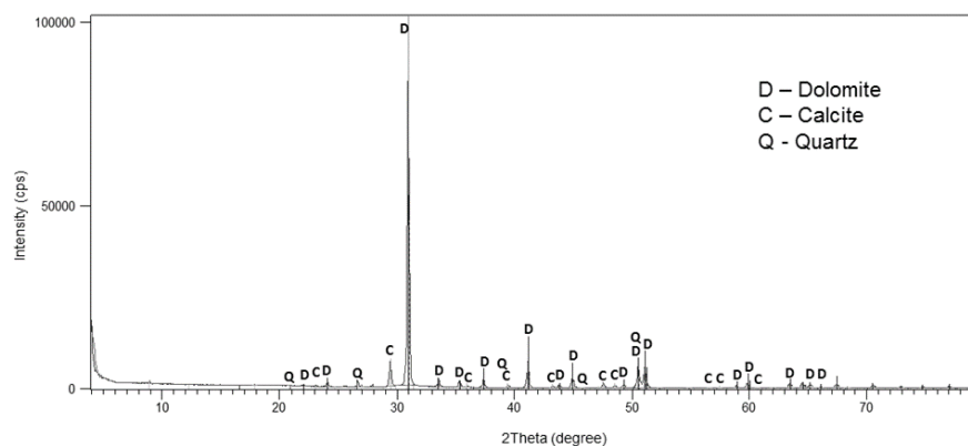
Fig. 1: XRD pattern of natural dolomite from Vrchlabi, Czech Republic
