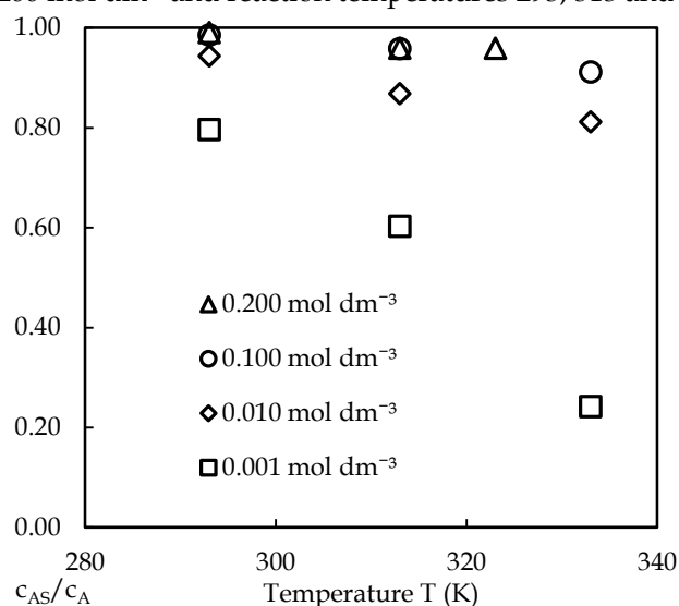
Fig. 8. Effect of temperature and nitric acid concentration on the c_{AS}/c_A ratio
