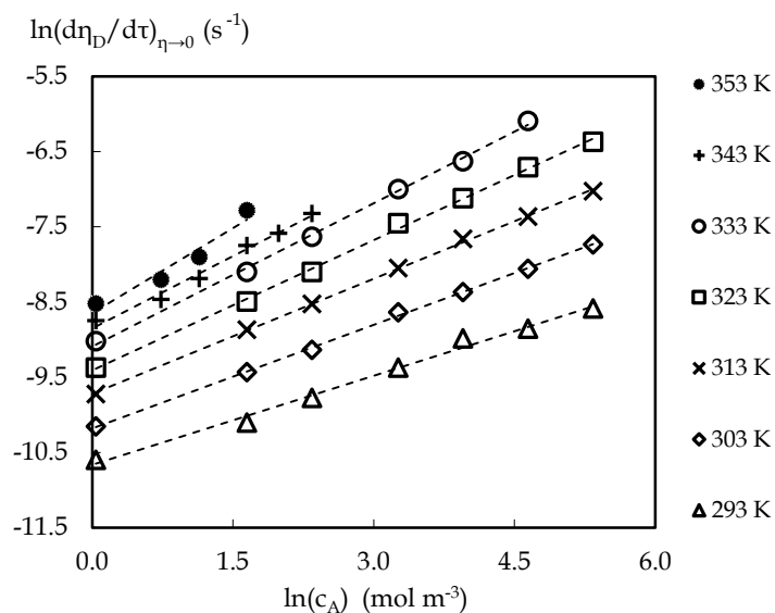
Fig. 6. Evaluation of the values of apparent reaction order for the studied reaction temperatures
