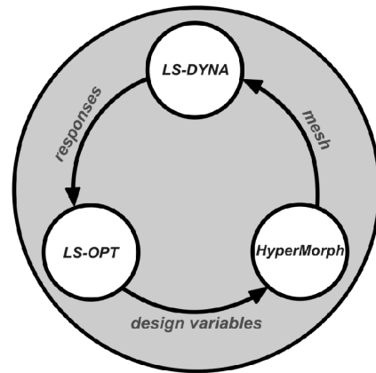
Fig. 2. Optimization toolchain
