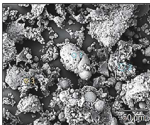
a. SEM image of geopolymer PW/GEO
