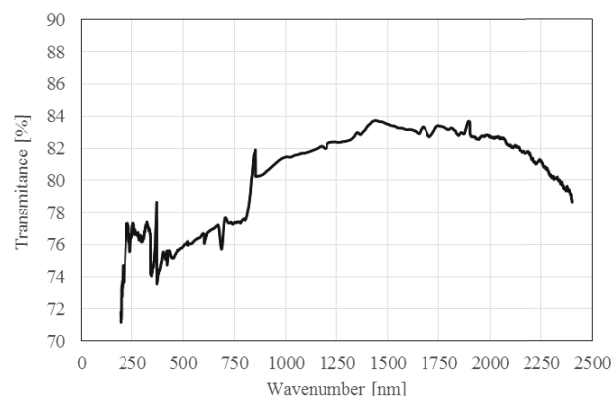
b. UV-VIS-NIR spectra of geopolymers PB/GEO
