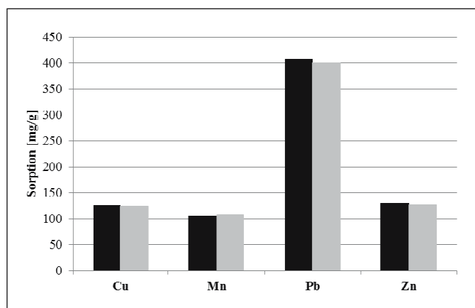
a. Participation of sorption mechanisms on the PW/GEO for the tested ions for initial metal concentration 0.01\text{ mol/dm}^3 (color black – ion exchange, color grey – chemisorption)
