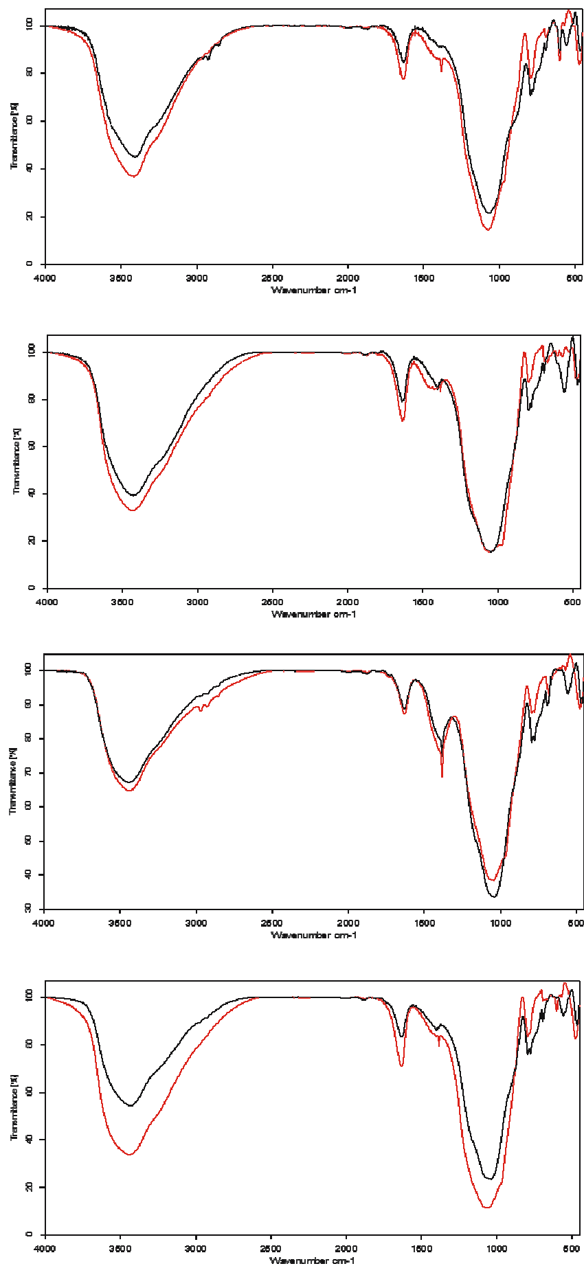
Fig. 7. FT-IR spectra after sorption the tested ions: a) Zn^{2+} , b) Mn^{2+} , c) Cu^{2+} , d) Pb^{2+} for initial metal concentration 0.01 \text{ mol/dm}^3 by geopolymers PB/GEO (line red) and PW/GEO (line black)
