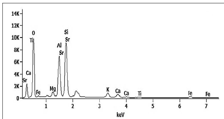
b. EDS analysis of biomass ash
