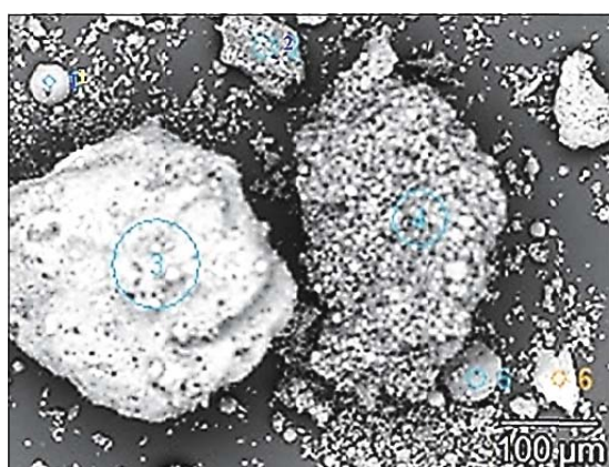
a. SEM image of coal ash
