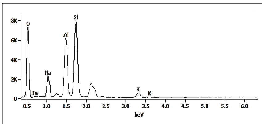
b. EDS analysis of geopolymer PW/GEO
