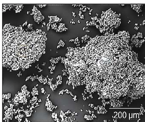
a. SEM image of geopolymer PB/GEO
