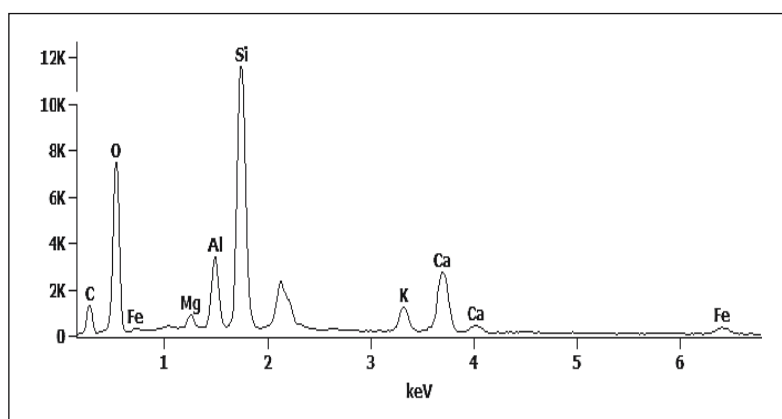
b. EDS analysis of coal ash
