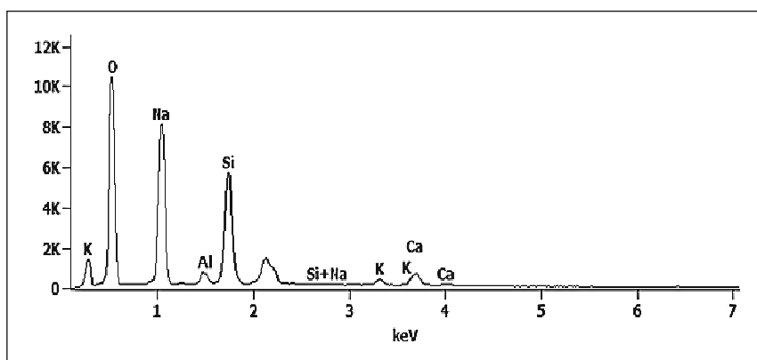
b. EDS analysis of geopolymer PB/GEO
