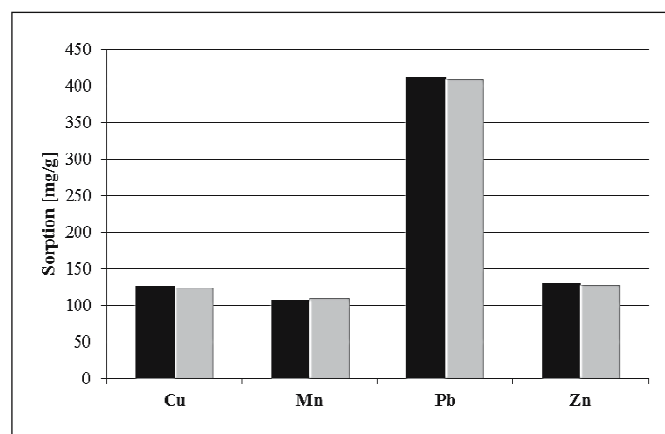
b. Participation of sorption mechanisms on the PB/GEO for the tested ions for initial metal concentration 0.01\text{ mol/dm}^3 (color black – ion exchange, color grey – chemisorption)
