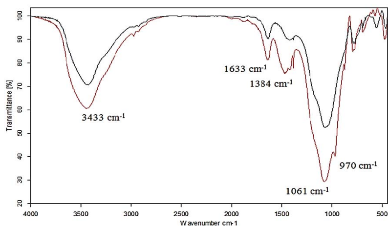
Fig. 5. FT-IR spectra of geopolymers; PW/GEO – color black and PB/GEO – color red
