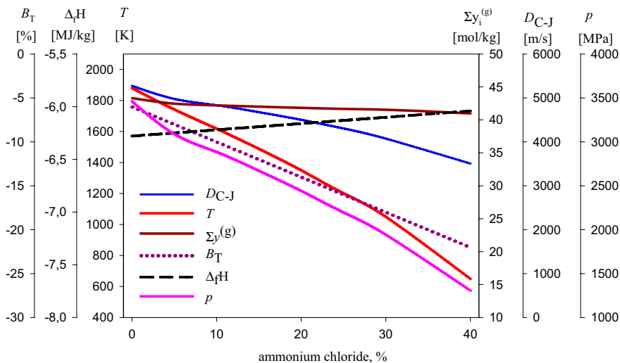
Figure 8. The dependence of the explosion parameters upon the ammonium chloride content in emulsion explosives based on the matrix M-2.
