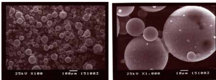
Figure 4. SEMs of the glass microballoons employed in the investigated explosives.
