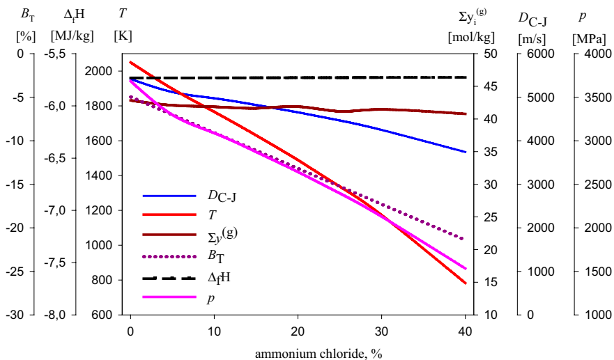
Figure 6. The dependence of the explosion parameters upon the ammonium chloride content in emulsion explosives based on the matrix M-1.
