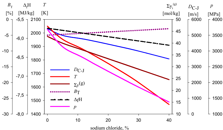
Figure 5. The dependence of the explosion parameters upon the sodium chloride content in emulsion explosives based on the matrix M-1.
