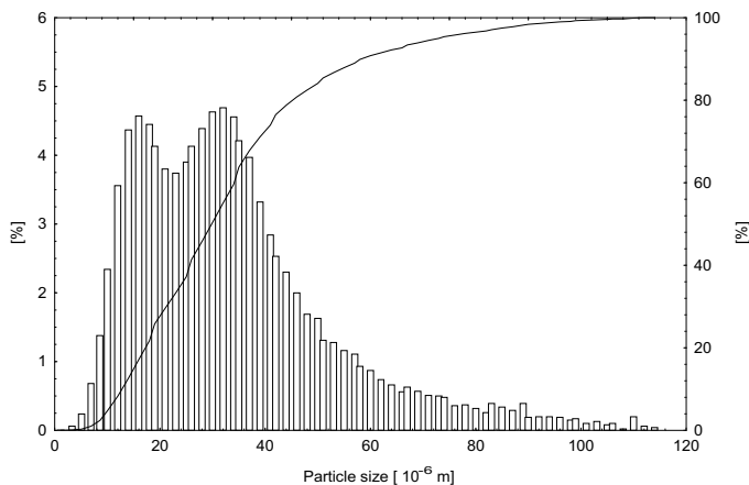
Figure 3. Particle size distribution of the glass microballoons.
