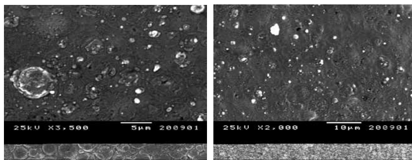
Figure 2. SEMs of matrix M-2.
