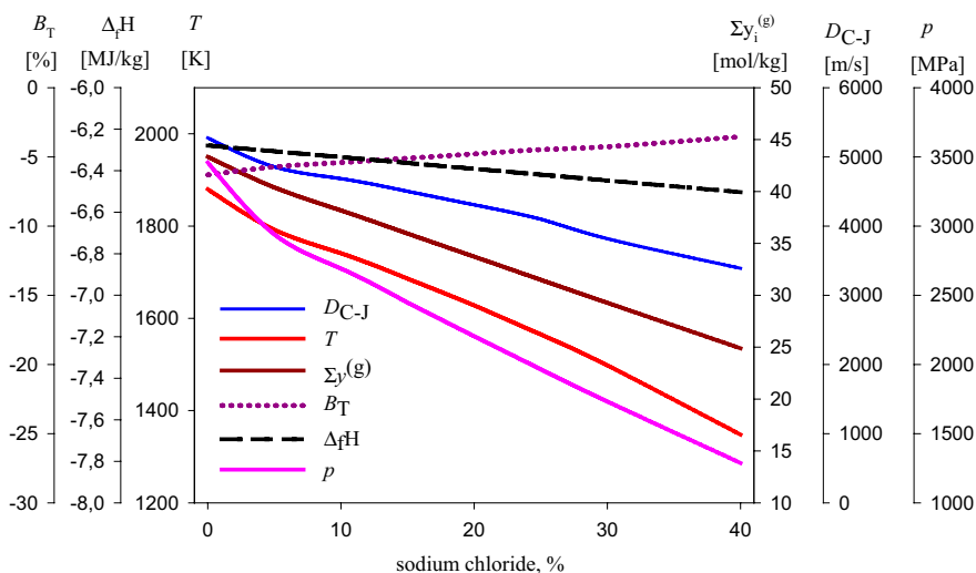
Figure 7. The dependence of the explosion parameters upon the sodium chloride content in emulsion explosives based on the matrix M-2.
