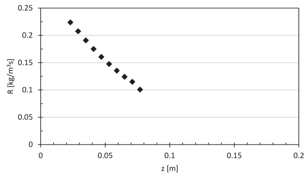
Figure 7: Drying rate.
