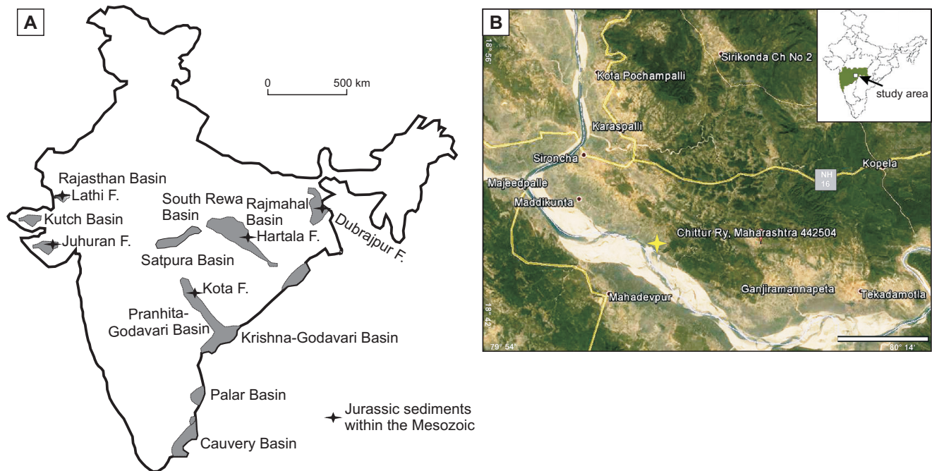
Fig. 1. A. Distribution of Mesozoic sedimentary basins in India, showing the Jurassic successions; B. Location map of Kota-Chittur area showing the fossil site
