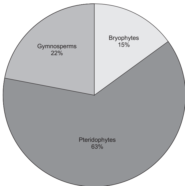
Fig. 3. Micro-floral diversity pattern of various taxonomic groups in the Kota-flora
