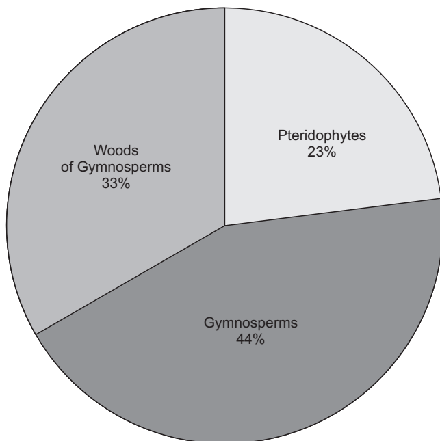
Fig. 2. Macro-floral diversity pattern of various taxonomic groups in the Kota-flora
