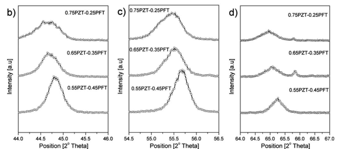
Fig. 2. XRD patterns for synthesized PZT-PFT type powders
