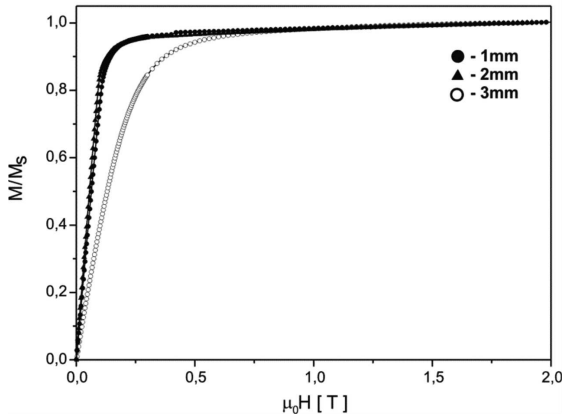
Fig. 5. Reduced magnetization curves for samples of amorphous Fe_{36}Co_{36}B_{19}Si_5Nb_4 alloy in the form of rods of 1 mm, 2 mm, and 3 mm diameters
