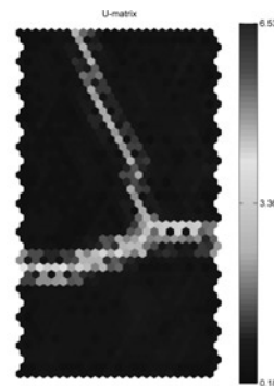
Fig. 6. Distance matrix for SOFM with 24 input features
