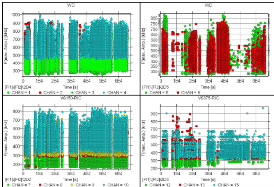
Fig. 10. Graphs of frequency values for the maximum amplitude of the signals ( F(\text{max. Amp.}) [kHz]), as the functions of time, for the entire period of testing of the bushing type MB58 [6, 22]
