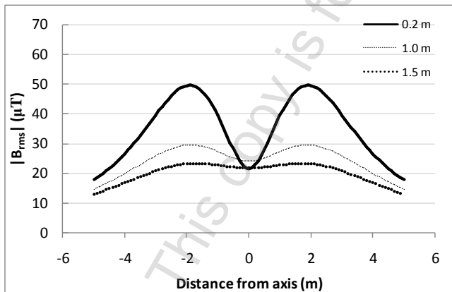
Fig. 2. Magnetic flux density distribution for the best combination
