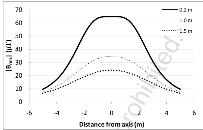
Fig. 3. Magnetic flux density distribution for the worst combination
