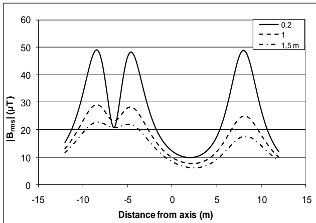
Fig. 6. Distribution of magnetic flux density with outage of one cable group
