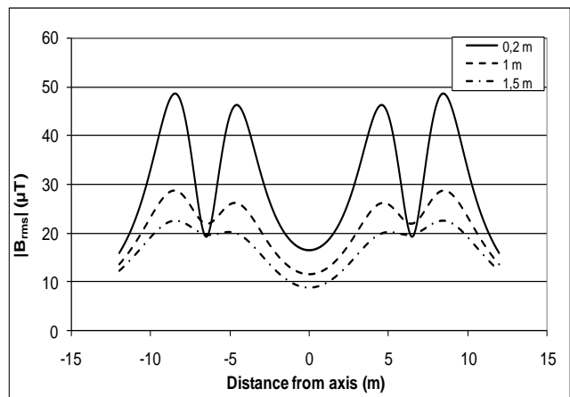
Fig. 5. Distribution of magnetic flux density for normal operation
