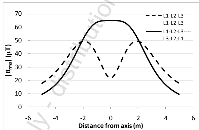
Fig. 4. Magnetic flux density distribution for the best and the worst combination at 0.2 m
