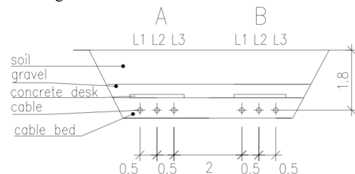
Fig. 1. The cable distribution in the trench
