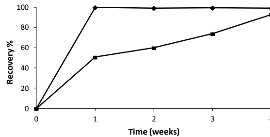
Fig. 13. Copper recovery as a function of (◆) biological or (■) chemical leaching time
