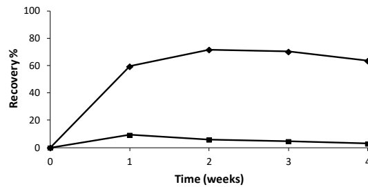
Fig. 9. Tin recovery as a function of time of (◆) biological and (■) chemical leaching
