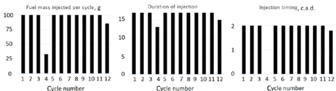
Fig. 4. Fuel injection control maps, which are used to examine the effects of an irregularity in fuel injection
