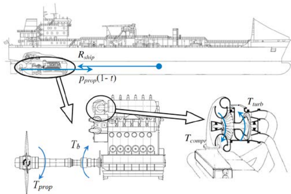
Fig. 3. Decomposition of the ship's propulsion system dynamics system
