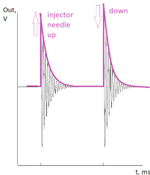
Fig. 2. Amplitude demodulation of high-frequency injector signals [18]
