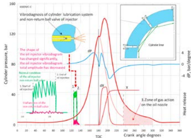
Fig. 7. Vibration diagram for the cylinder lubrication injector, combined with a P(deg) diagram
