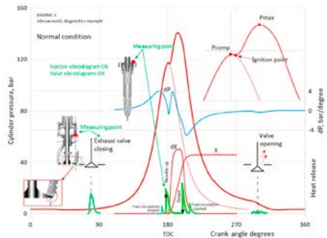
Fig. 1. Example of diagnostics data, including superimposed diagrams of the in-cylinder gas pressure (red line) and the processed vibration sensor signals from the fuel injector and exhaust valve [18]
