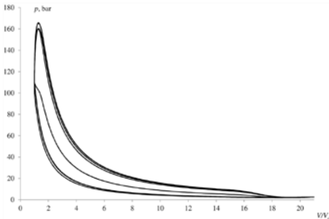
Fig. 6. Cycle variations under irregular fuel injection conditions
