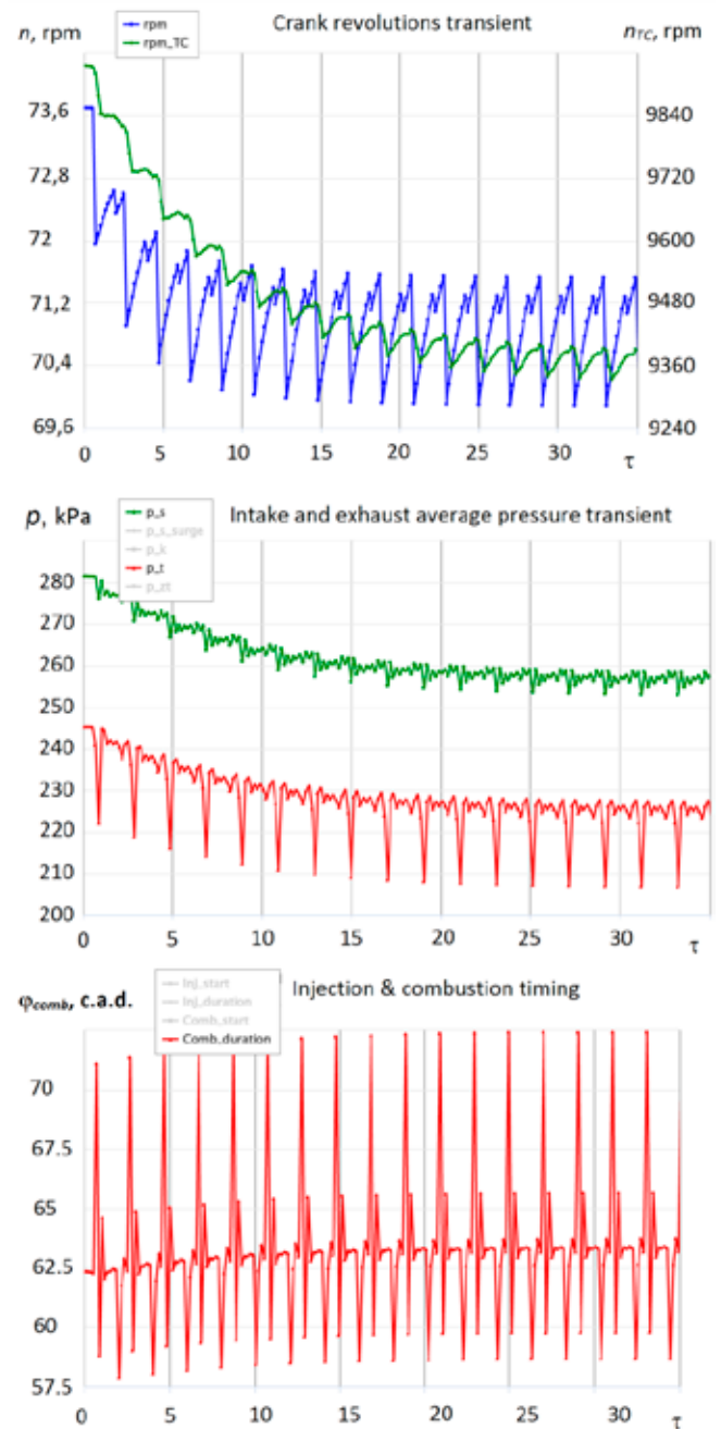
Fig. 5. Results for transient engine operation under a fuel injection irregularity
