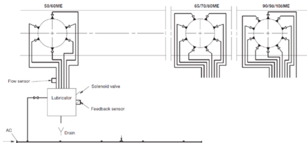
Fig. 8. Cylinder lubricator system for ME engines [23]
