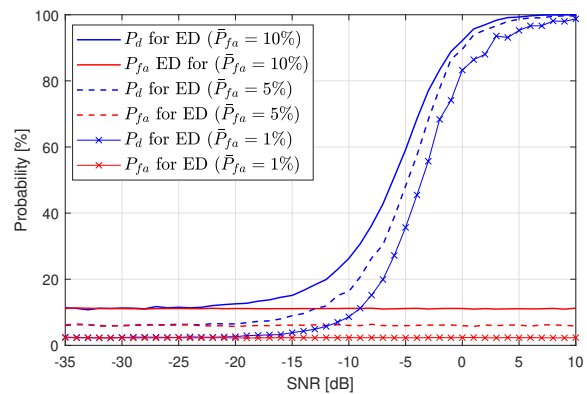
Fig. 3. ED results comparison for different \bar{P}_{fa} values.
