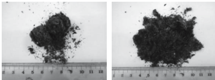
Fig. 3. Ash from burning fuel based on oat straw with the admixture of shredded polyethylene (by M. Czop)
