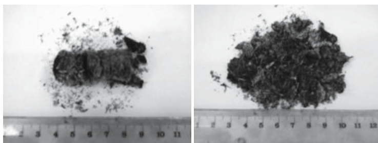
Fig. 4. Ash from burning fuel based on oat straw with the admixture of not shredded polyethylene (by M. Czop)
