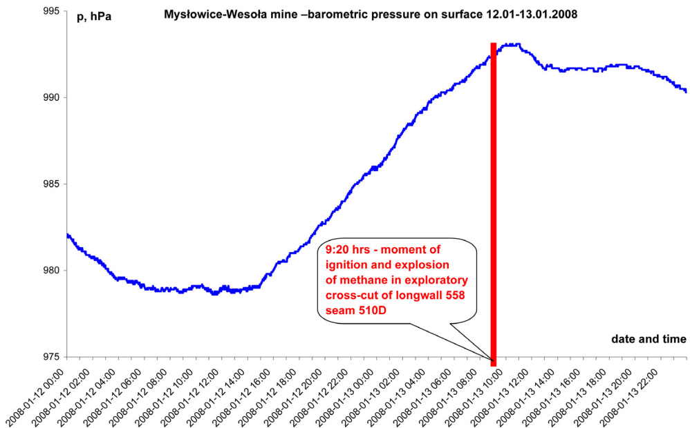
Fig. 14. Changes in barometric pressure at the mine surface during the time preceding the ignition and explosion of methane on 13.01.2008 at the Mysłowice-Wesola coal mine
