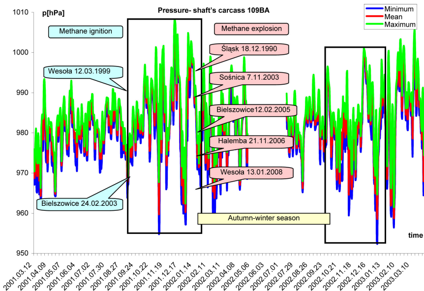
Fig. 7. Ignitions and explosions of methane in the gob relative to seasonal changes in pressure
