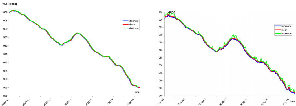
Fig. 5. Weekly barometric pressure changes at the mine surface and underground
