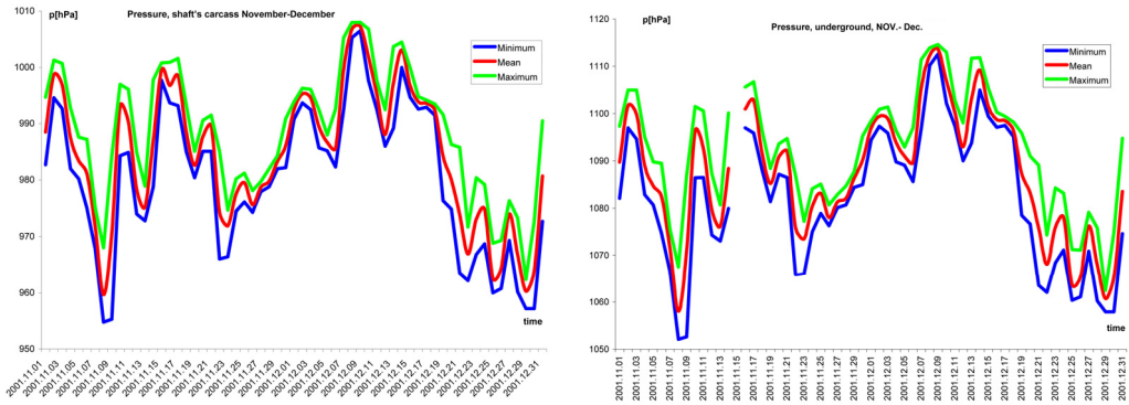
Fig. 4. Pressure changes at the surface and underground during late autumn
