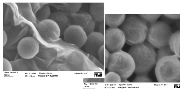
Fig.1. SEM image of the structure of a PVDF/acetone/toluene/GR composite.
