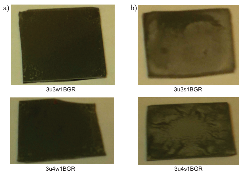
Fig. 5. Images showing the quality of the graphene/PVDF composite layers obtained by centrifugation (left pictures) and sedimentation (right pictures).
