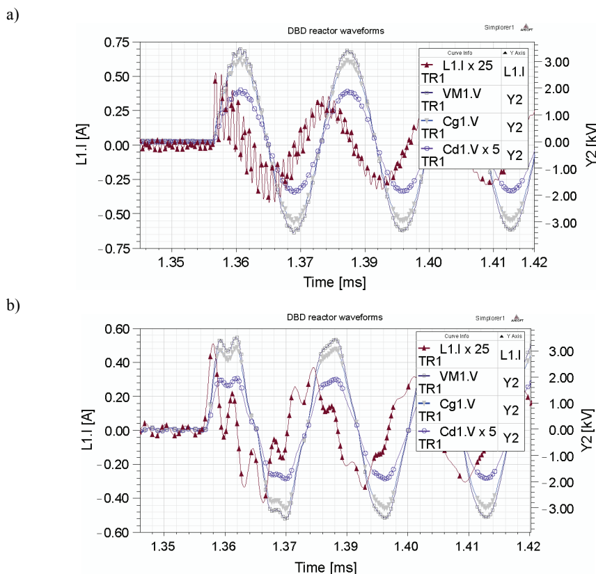
Fig. 4. Converter – reactor waveforms: a) basic configuration without series inductance; b) with series, saturable inductor
