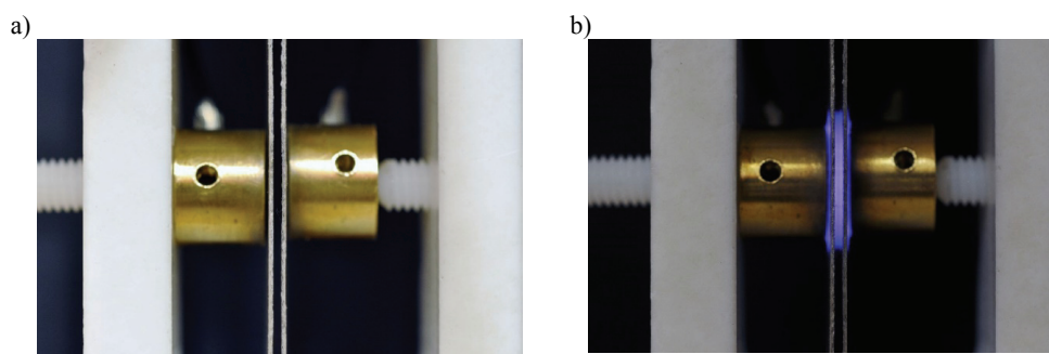
Fig. 8. Camera imaging of the light intensity: a) discharge cell, b) DBD discharge with saturable inductor
