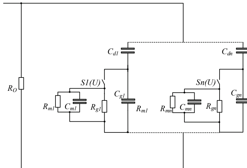
Fig. 3. DBD reactor model
