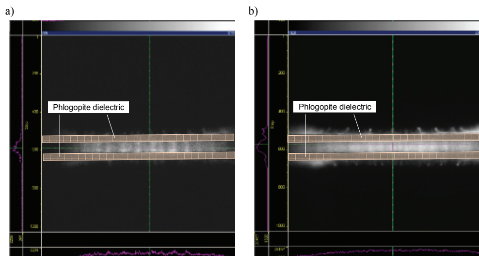
Fig. 9. iCCD camera imaging of the light intensity: a) no additional inductance, b) saturable inductor
