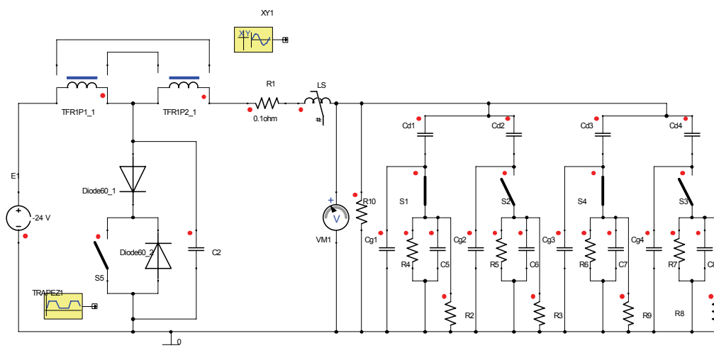
Fig. 2. Simulation model of pulsed power supply and a DBD reactor model
