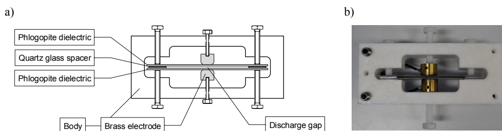
Fig. 5. DBD discharge cell used for examinations: a) basic configuration; b) constructed discharge cell
