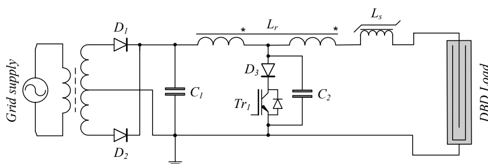
Fig. 1. Topology of a pulsed power electronic converter used for experiments
