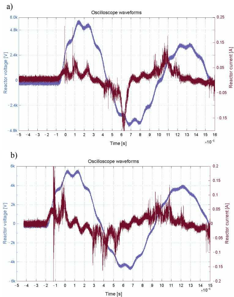
Fig. 7. Recorded oscilloscope waveforms in case of a) no additional inductance, b) saturable inductor
