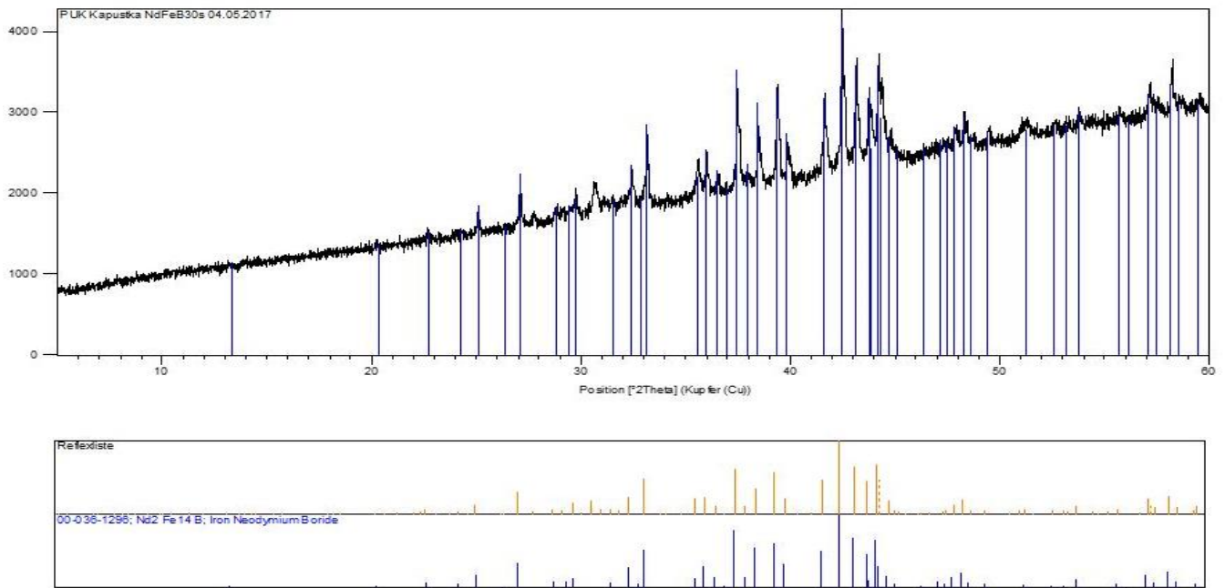
Fig 1. X-ray spectrum for recovered magnets from electric motors
