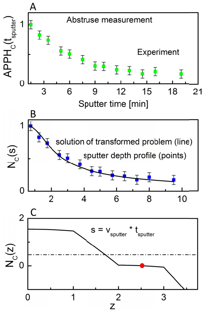
Fig. 2. Results for the desorbed carbon/passive layer on an NiTi substrate. The experimental data (points) are illustrated in A. Conversion of the sputter time into depth ( s \approx v_{\text{sputter}} t_{\text{sputter}} , where v_{\text{sputter}} \cong 0.5 carbon monolayer/min) in the sputter depth profile (points) is plotted in B. The fitted function (solid line) gives the following parameter values: A \cong 0.87 , \tilde{E} = 0.01 eV, V_o = 0.09 eV, M = 1 kg ^{-1} , C = 1.25 , \tau_C = 1 , \alpha = 1.6 and i = 1, 2, 3, \dots, 9 . Parameter A is a dimensionless constant, \tilde{E} is the total energy of Auger electron, V_o is the potential energy of this electron, M is the sum of the inverse mass of particles (electrons), C and \alpha is the dimensionless constant and \tau_C is the source position of the Auger electron emission from the carbon layer. The interpolation of Equation (8) was used to receive Equation (11) with the help of nonlinear fit as given in Microcal Origin. The solution function of Equation (5) is shown in panel C (see Equation (12)). The large dots denote the critical value of the solution between the positive and negative signs
