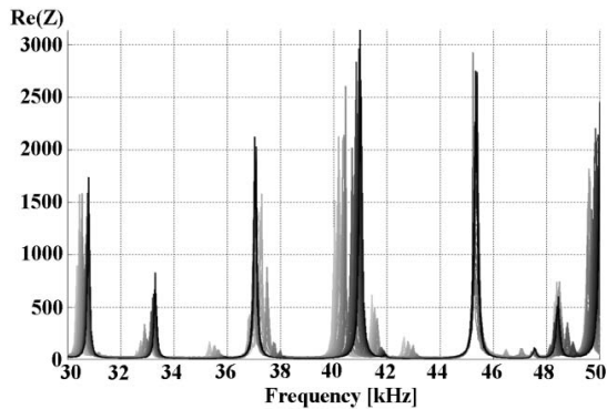
Fig. 9. Point FRFs for growing damage size (black curve refers to the nominal FE model)
