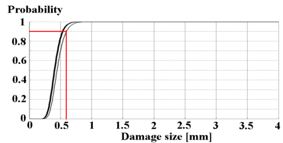
Fig. 11. Probability of damage detection and related confidence interval
