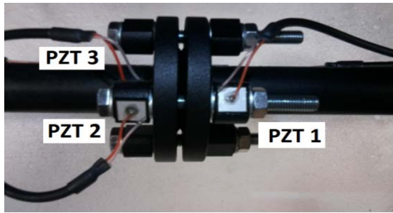
Fig. 2. Monitored pipeline section
