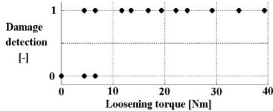
Fig. 6. Ordered damage cases
