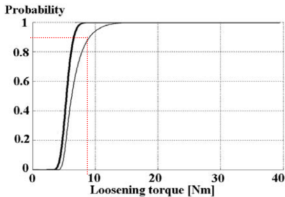
Fig. 7. Probability of detection
