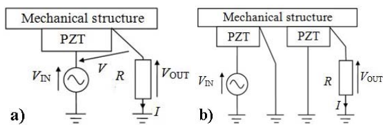
Fig. 1. Measurement of point FRF (a), and transfer FRF (b) of electromechanical impedance
