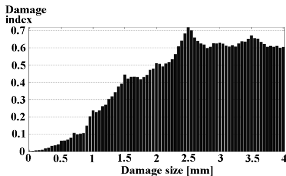
Fig. 10. Relationship between notch depth and damage index
