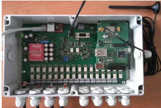
Fig. 3. Developed Data Acquisition Unit
