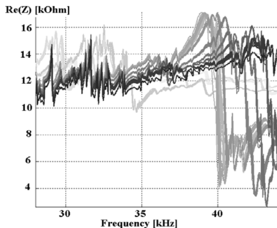
Fig. 4. FRFs for real parts of electromechanical impedance (black curve refers to the nominal healthy state)
