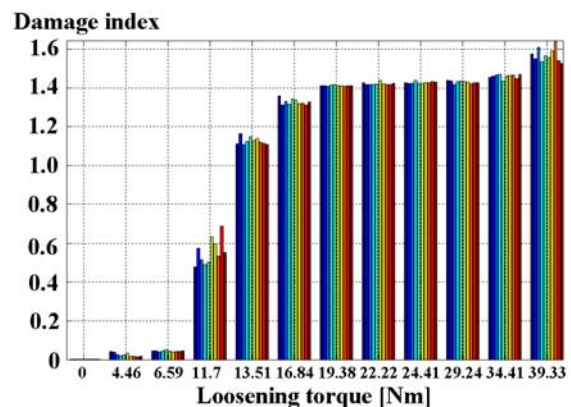
Fig. 5. Relationship between the loosening torque and the damage index
