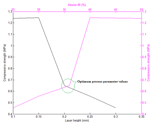
Fig. 6. Compressive strength against interior fill and layer height
