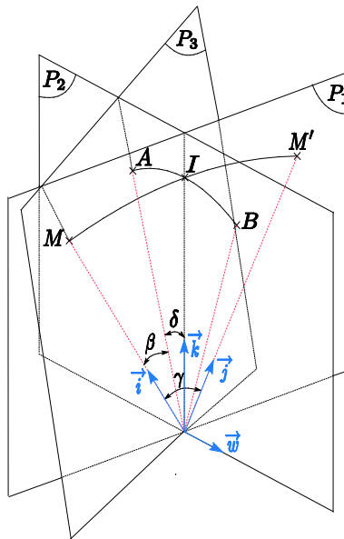
Figure 1. Main planes to define the meshing
