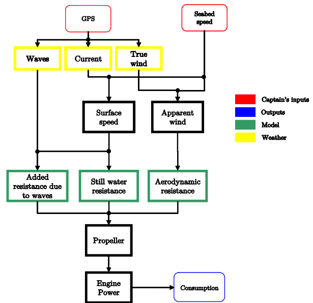
Figure 5. Scheme calculation of the consumption
