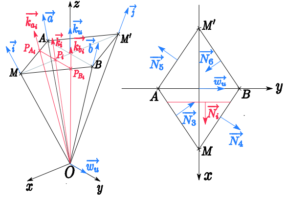
Figure 2. Definition of planes P_i
