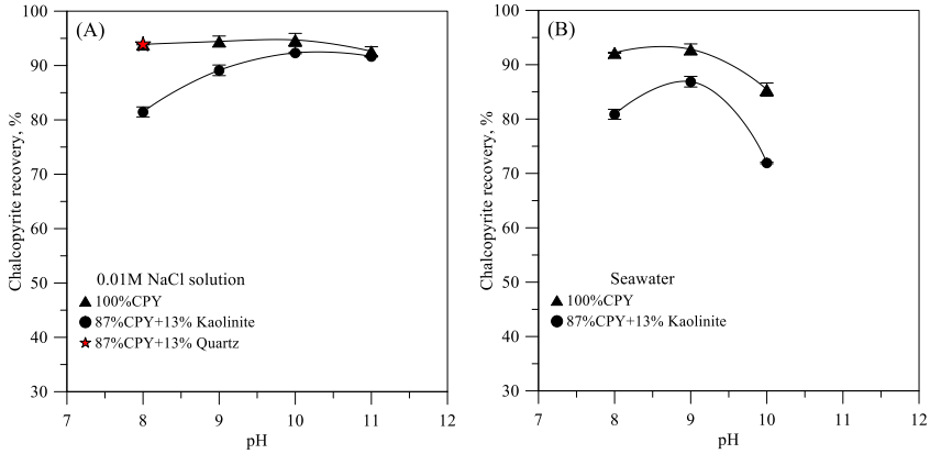
Fig. 2. Effect of the presence of kaolinite on the recovery of chalcopyrite as a function of pH in (A) 0.01 M NaCl solution and (B) seawater. Conditions: 40 ppm PAX, 25 ppm MIBC. CPY denotes chalcopyrite
