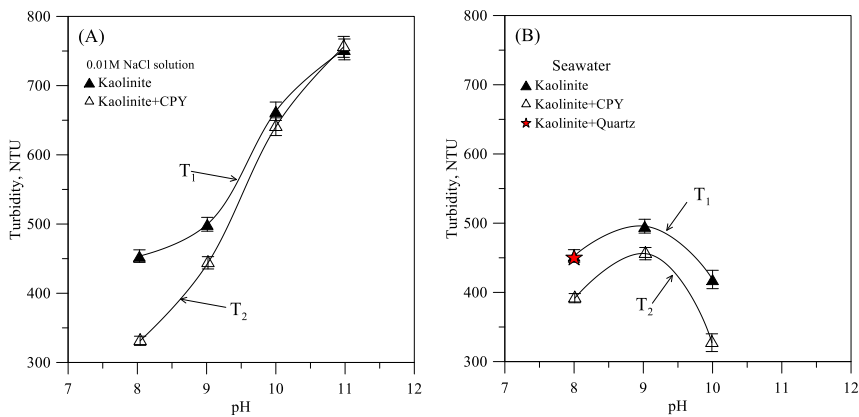
Fig. 6. Turbidity of suspensions of kaolinite, and 13% kaolinite + 87% chalcopyrite prepared with (A) 0.01 M solutions of NaCl and (B) seawater (for definitions of T 1 and T 2 see Figure 1)
