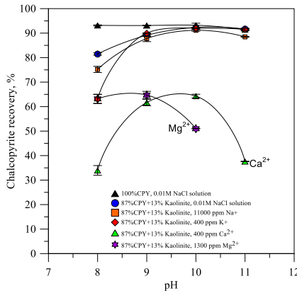
Fig. 3. Effect of the presence of kaolinite on the recovery of chalcopyrite as a function of pH in solutions that contain 11000 ppm \text{Na}^+ , 400 ppm \text{K}^+ , 400 ppm \text{Ca}^{2+} , and 1300 ppm \text{Mg}^{2+} . Conditions: 40 ppm PAX, 25 ppm MIBC
