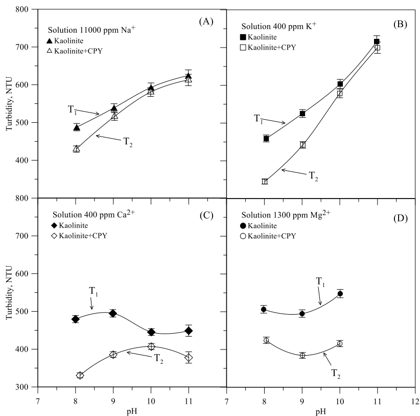
Fig. 7. Turbidity of suspensions of kaolinite, and 13% kaolinite+87%chalcopyrite suspension prepared with solutions containing 11000 ppm Na + , 400 ppm K + , 400 ppm Ca 2+ , and 1300 ppm Mg 2+
