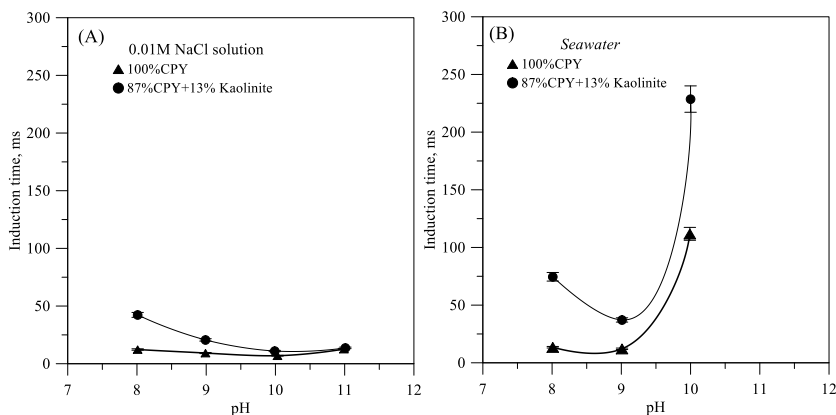
Fig. 4. Effect of the presence of kaolinite on the induction time in (A) 0.01 M NaCl solution and (B) seawater
