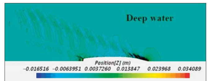
b) wave patterns at V=1.199 m/s
