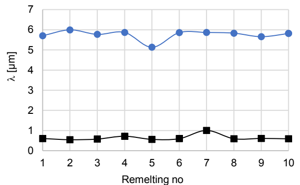
Fig. 4. Arrangement of Al 2 O 3 particles and precipitates in the composite metal matrix vs number of remelting operations (squeeze casting)
