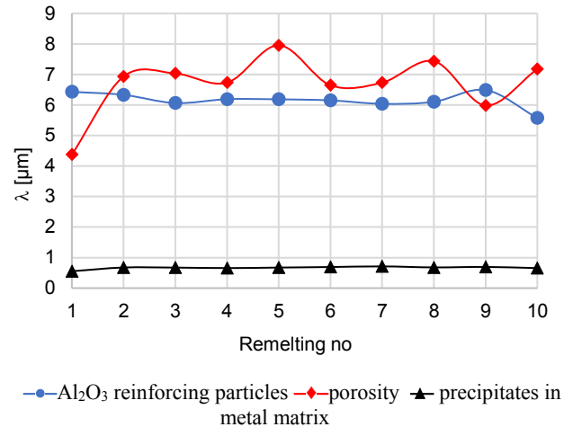
Fig. 3. Arrangement of Al 2 O 3 particles, pores and precipitates in the composite metal matrix vs number of remelting operations (gravity casting)
