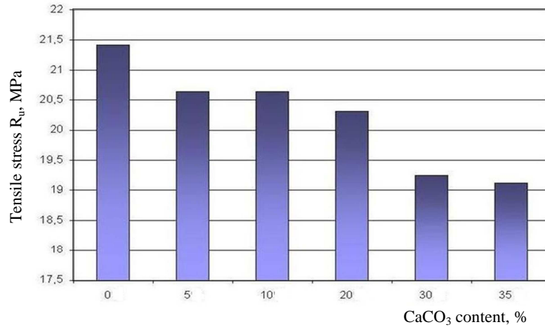
Fig. 1. Maximum tensile stress R_u versus \text{CaCO}_3 content
