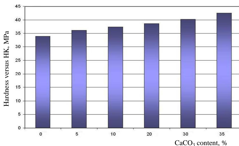
Fig. 3. Hardness versus \text{CaCO}_3 content
