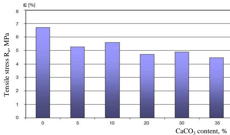
Fig. 2. Elongation at R_u versus \text{CaCO}_3 content
