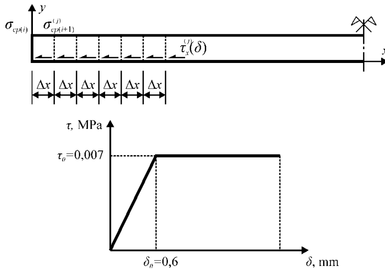
Figure 2.1. To the calculation of the pre-stress distribution
