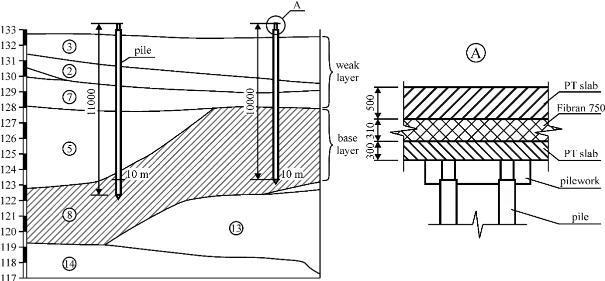
Figure 3.1. Geological survey's results and construction of foundation
