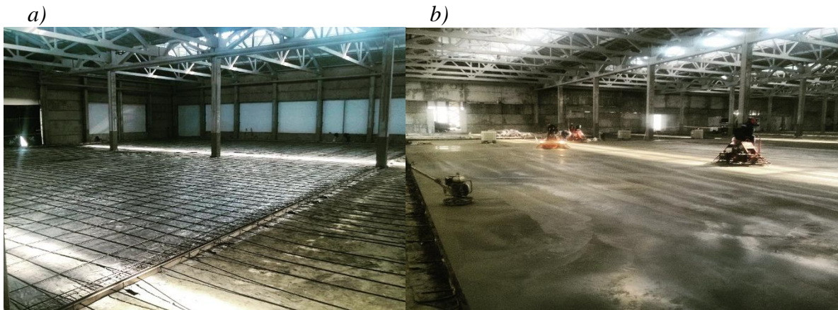
Figure 3.5. Tendon layout in formwork (a) and slab after concreting (b)
