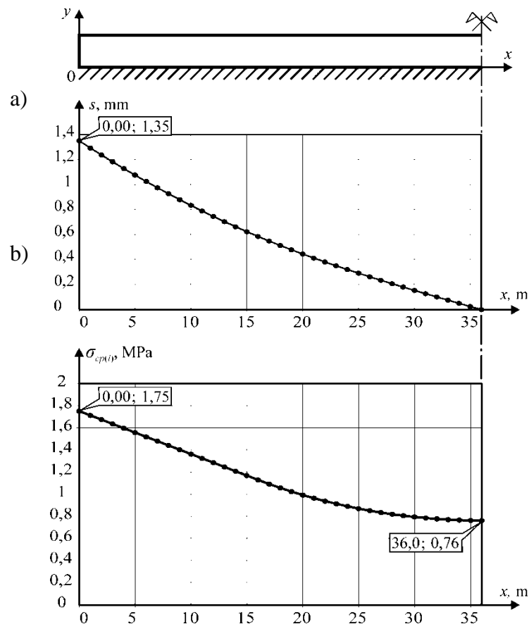
Figure 3.6. Displacements (slippage) (a) and pre-stress distribution (b) along the length of the slab (half of the length-symmetrically)
