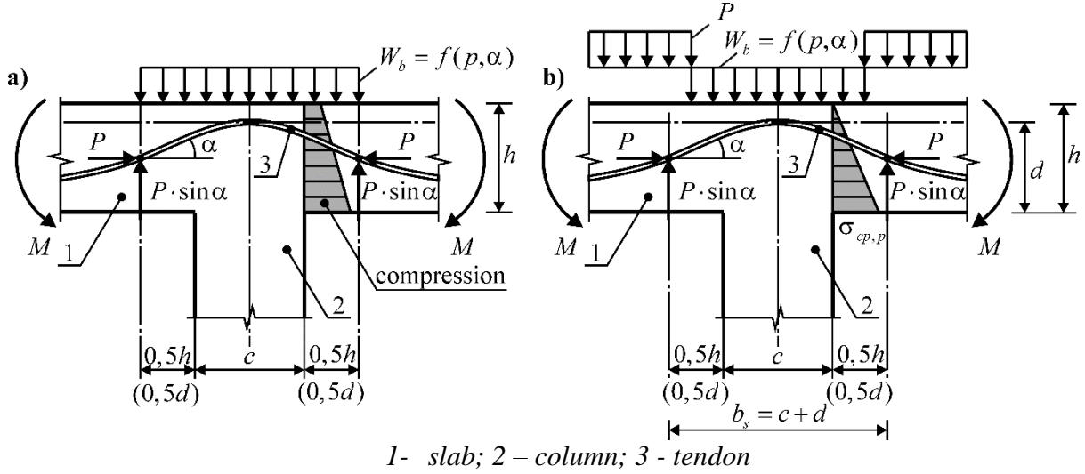
1- slab; 2 – column; 3 - tendon Figure 1.1. The scheme of forces for determining the vertical and horizontal component of the compression force (a) before the application of the vertical loads; (b) state of decompression
