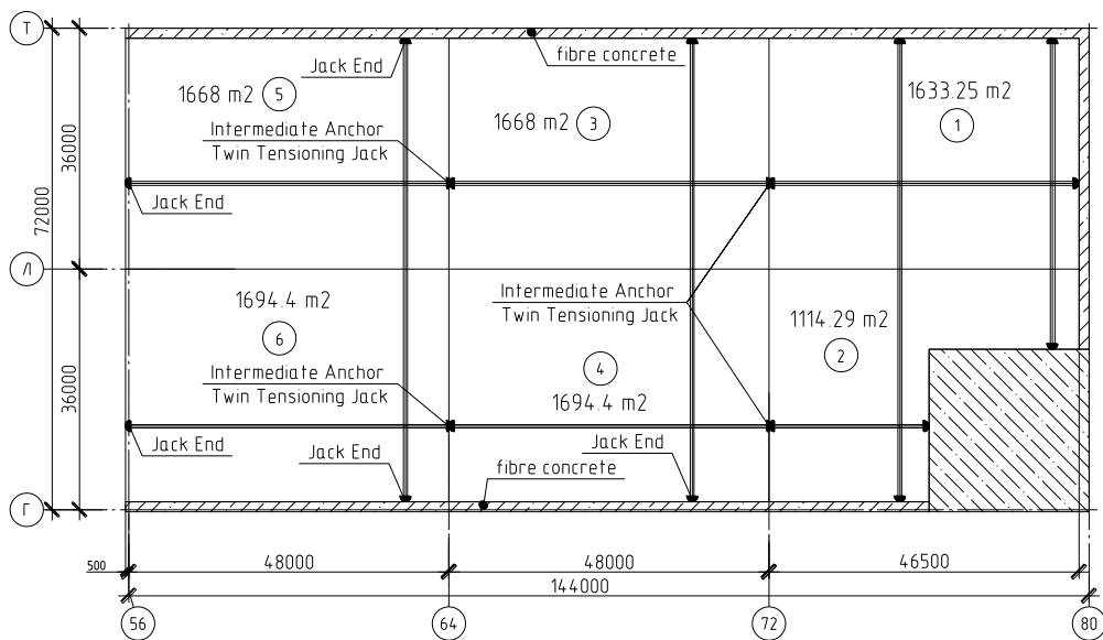
Figure 3.4. Slab plan with tendon profile
