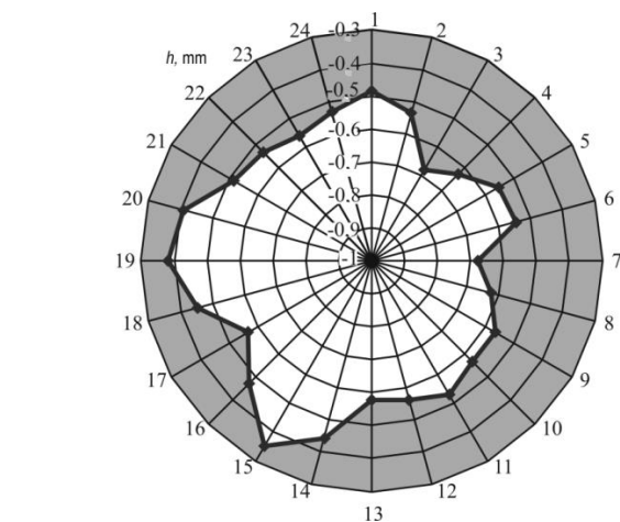
Fig. 5. Radial residual deformation (mm) on diameter of the shaft after testing on mechano-rolling fatigue ( N_{\Sigma} = 976100 cycles)
