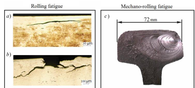
Fig. 2. Local damages - microcracks during wear peeling (a) and chipping (b) during rolling fatigue and photo of the fracture of railway rail from the transverse crack of mechano-rolling fatigue (c)
