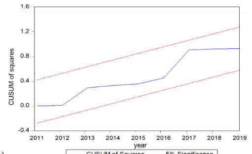
(a) (b) Fig. 3. CUSUM (a) and CUSUMSQ (b) for parameter stability tests of Model 2 in equation (12)
