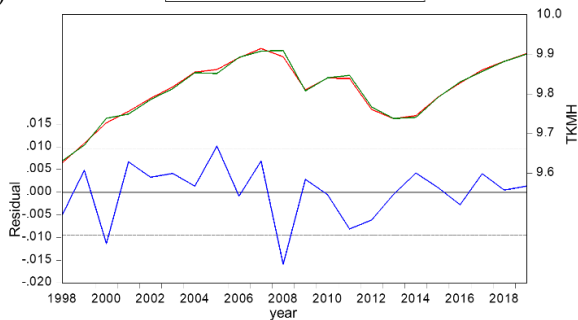
Fig. 4. Residual, actual and fitted time series for model 1 (a) and model 2 (b)
